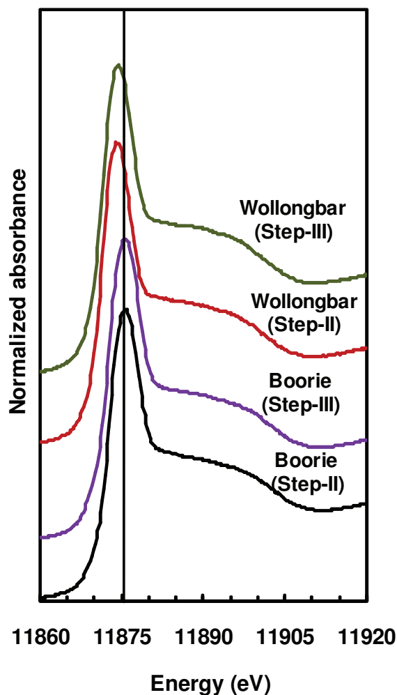
Figure 7.4 Arsenic K-edge XANES spectra for Boorie (black and purple lines) and Wollongbar (red and green lines) soil samples analysed after Step-II and Step-III of the SEP. The solid (–) line is drawn at 11875.7 eV represent the position of white line for arsenate ( \text{As}^{\text{V}} ).
