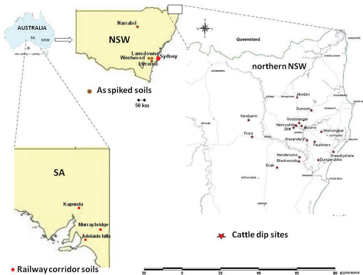
Figure 7.1 Locations of the As-contaminated cattle-dip sites, railway corridor and As spiked soil samples collected from New South Wales (NSW) and South Australia (SA) states of Australia.
