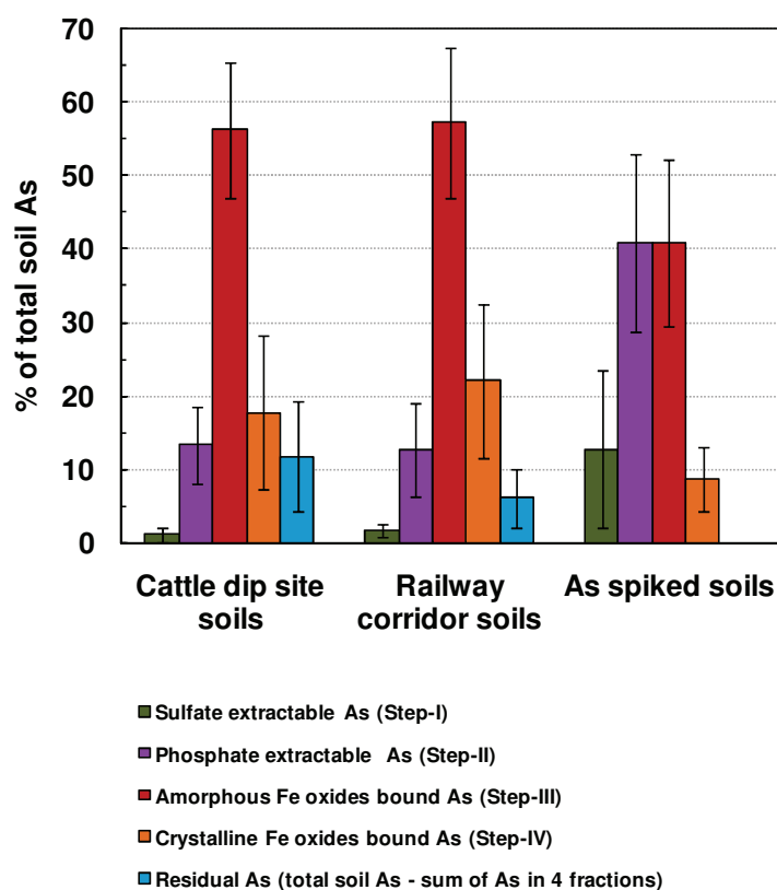
Figure 7.2 Sequential extraction procedure applied to the cattle-dip sites, railway corridor and As spiked soil samples ( n = 18, 3 and 11 , respectively). Means of each extracted fraction are presented as percent (%) of the total soil As concentration present in the contaminated and As spiked soils. The residual fraction of As was calculated by subtracting sum of the four fractions from the total As concentration in each of the soils. The bars represent \pm SD around the mean values.
