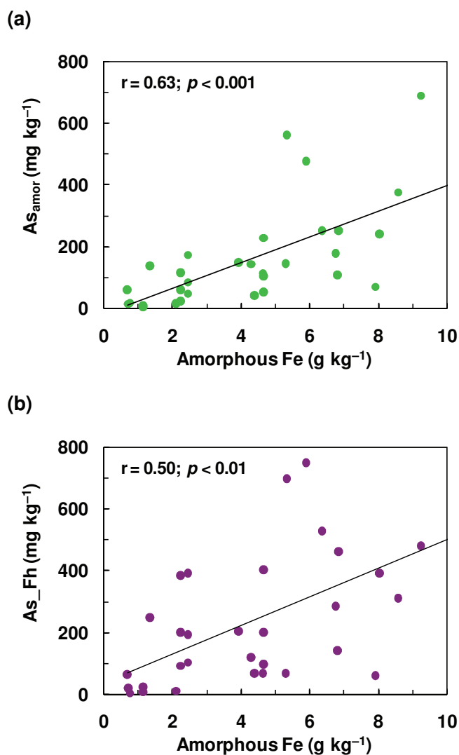
Figure 7.6 The relationship of amorphous (ammonium oxalate extractable) Fe concentration with the amorphous Fe oxides associated As in the studied soils determined using (a) SEP in Step-III, and (b) XANES spectroscopy.
