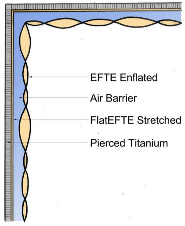
SCREEN SYSTEM AND STRUCTURE Exterior screen of Pierced Titanium (example 1) backed by EFTE. Interior screen enflated EFTE (example 2) with printed pattern to help control sun glare. Air barrier in the middle to control ventilation of building
