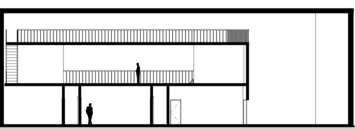
SECTION 2 1:200 Long section through building showing the double height garage which is open both sides for free flowing truck and car movement in the need of emergencies
