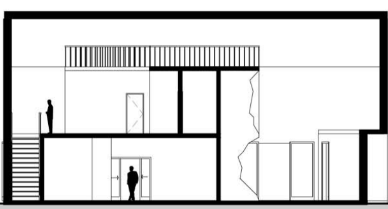
SECTION 1 1:200 Short section through building showing both sides of building open to experience the screen at both a close and detailed level and an overall view
