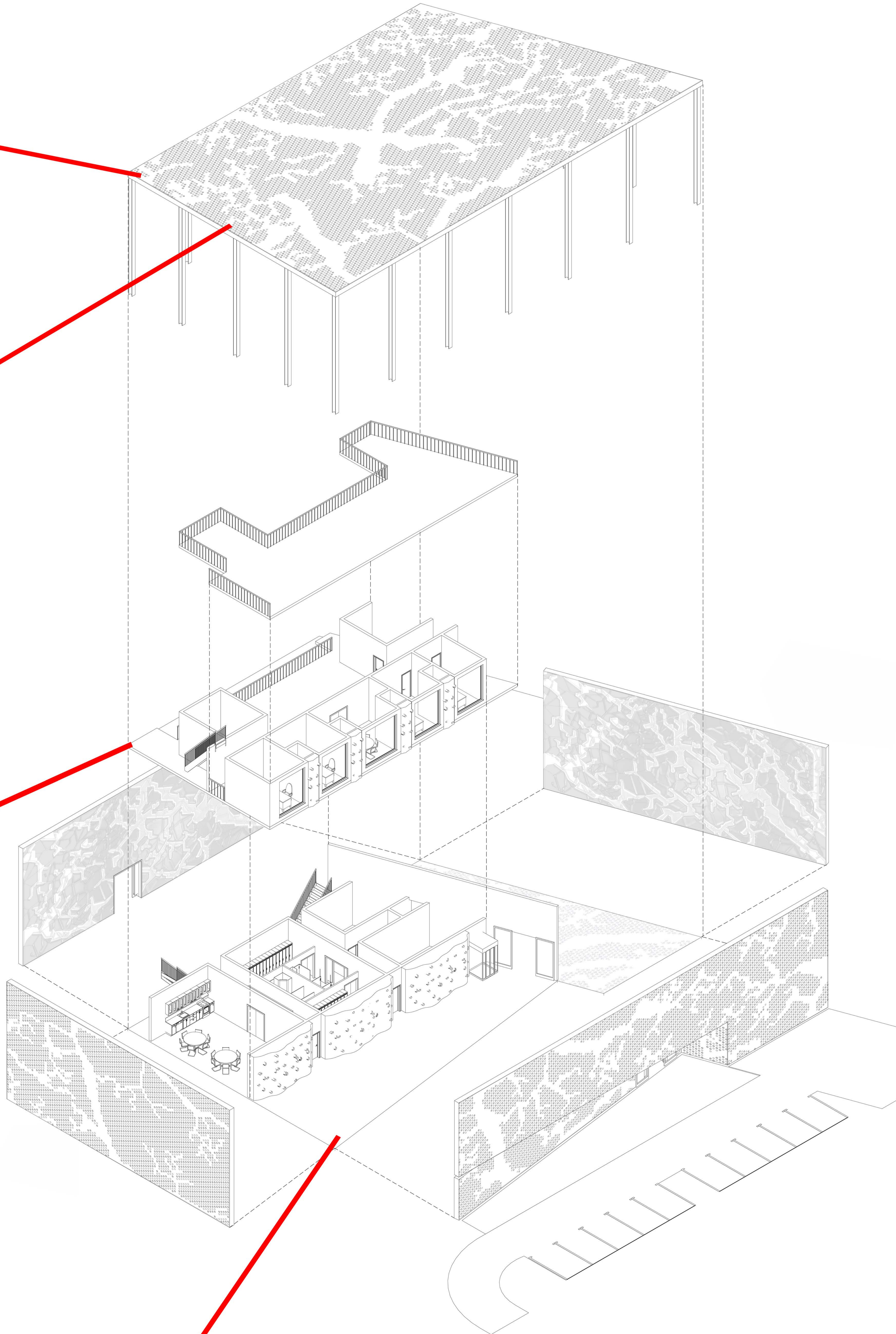
SCREEN SYSTEM AND STRUCTURE Exterior screen of Pierced Titanium (example 1) backed by EFTE. Interior screen enflated EFTE (example 2) with printed pattern to help control sun glare. Air barrier in the middle to control ventilation of building
