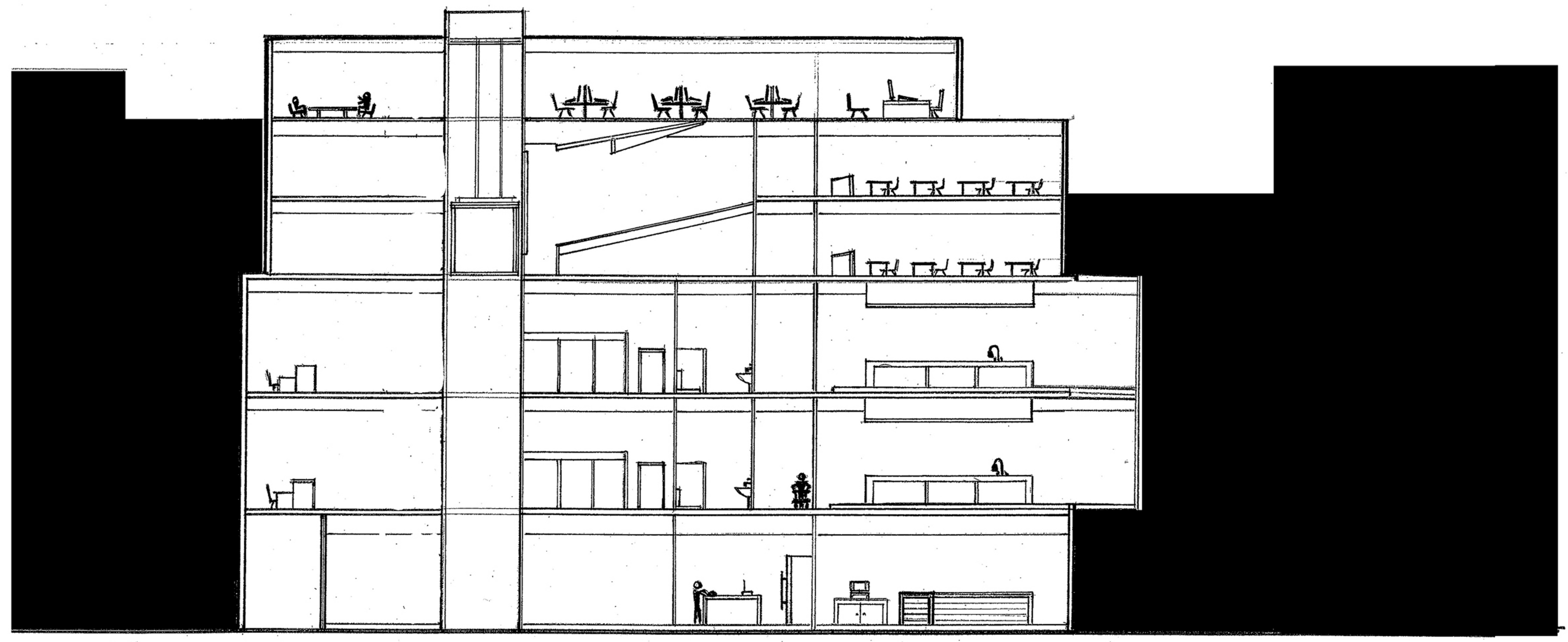
Section 1:200
