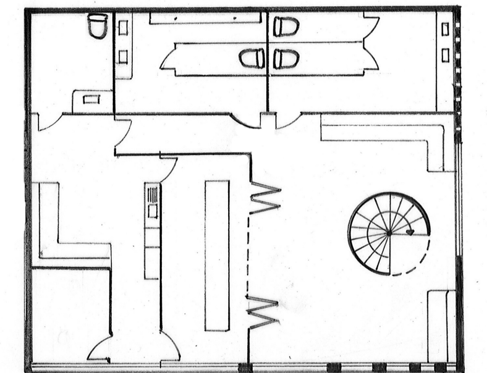
second floor 1:200
