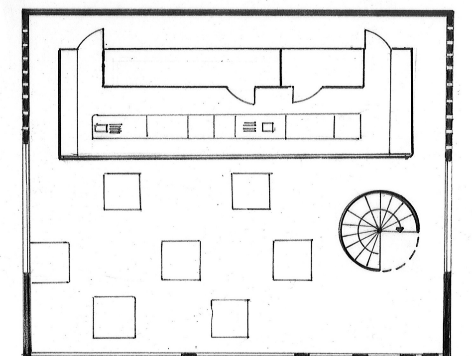
third floor 1:200
