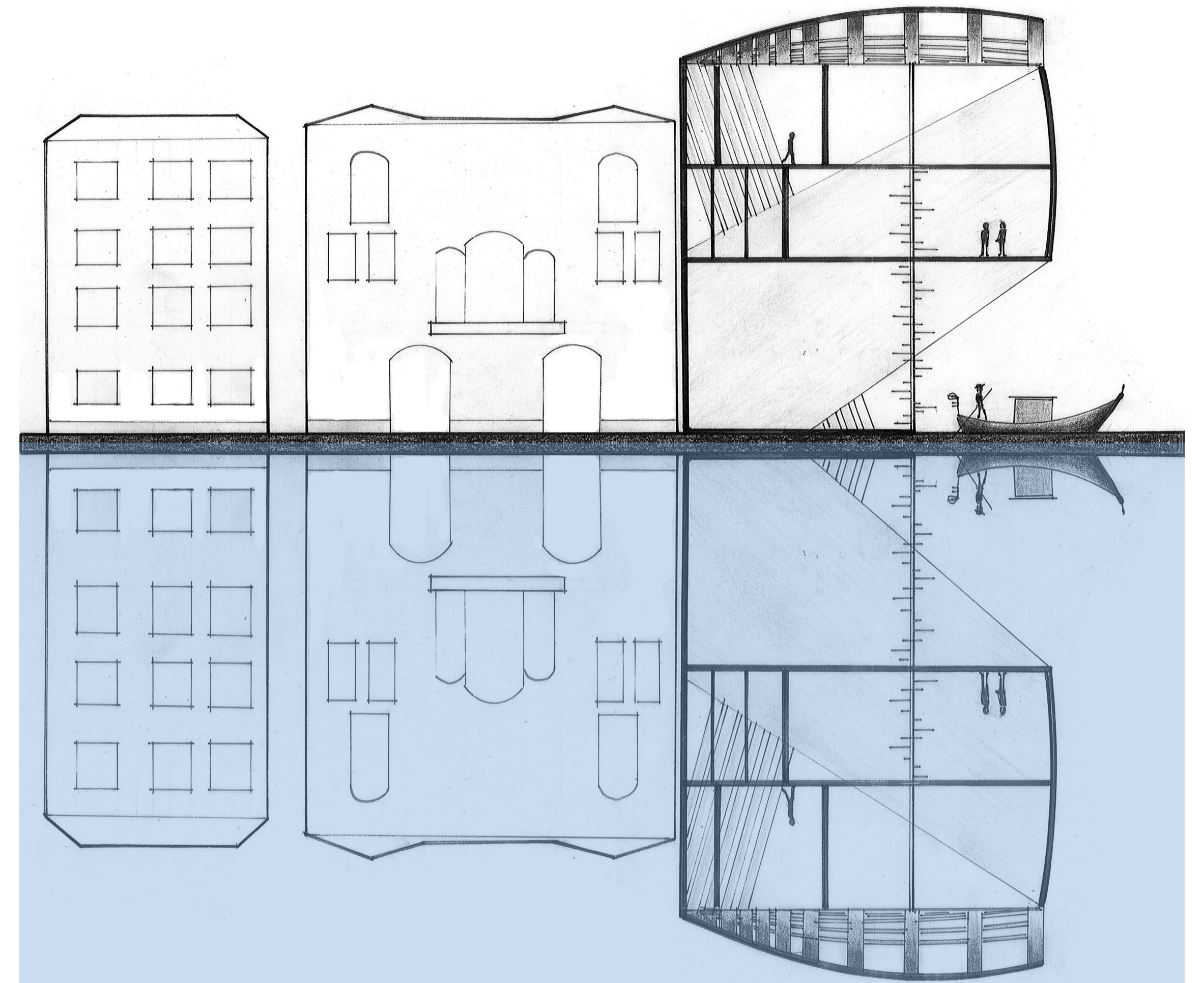
section 1:200
