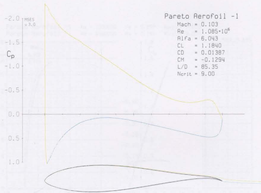
Figure 6.7: Pressure coefficient distribution and aerodynamic data for Pareto 01 for flight condition one [Slow-Cruise].
