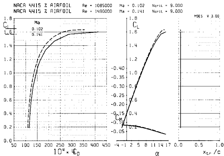
Figure 6.3: Polar computation for NACA 4415 aerofoil.
