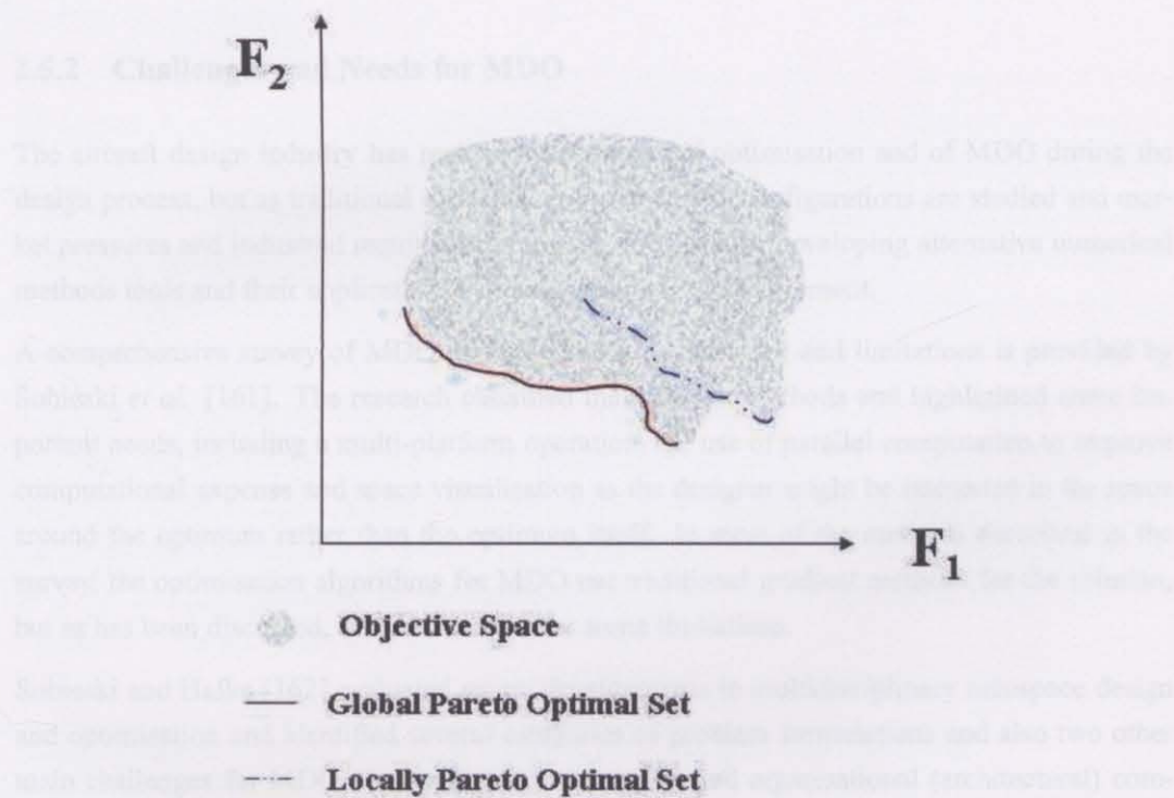
Figure 2.5: Locally and global Pareto optimal solutions.
