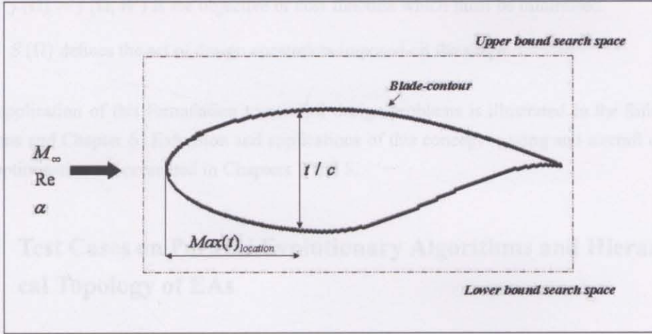
Figure 5.2: Two-dimensional section of an aerofoil wing.
