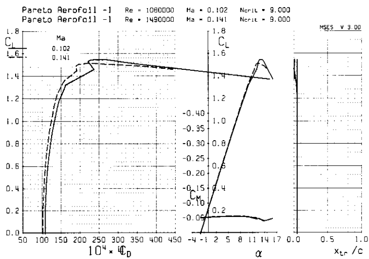
Figure 6.16: Polar computation for Pareto 01 aerofoil [ C_m Constrained].
