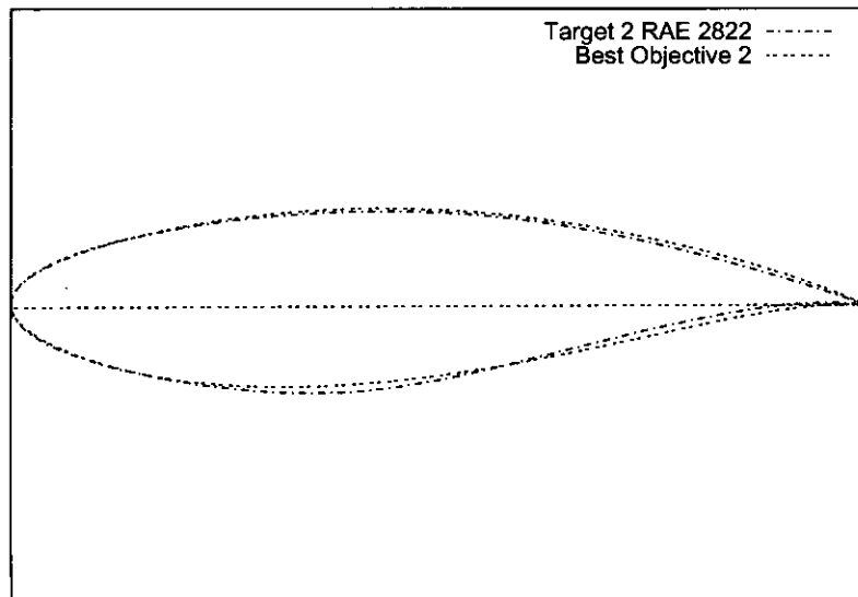
Figure 5.16: Target and computed geometries, multi-point aerofoil design, objective two.
