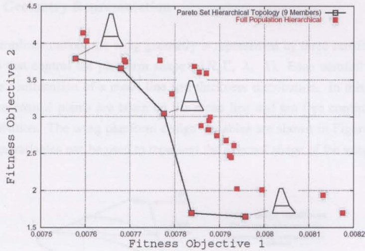
Figure 7.14: Pareto fronts and wing planforms.
