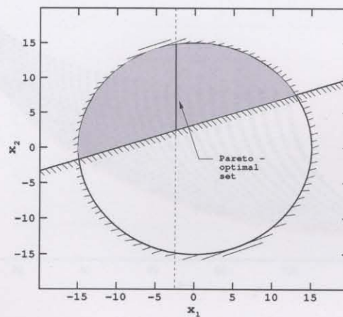
Figure 4.8: Decision variables space for constrained problem SRN.
