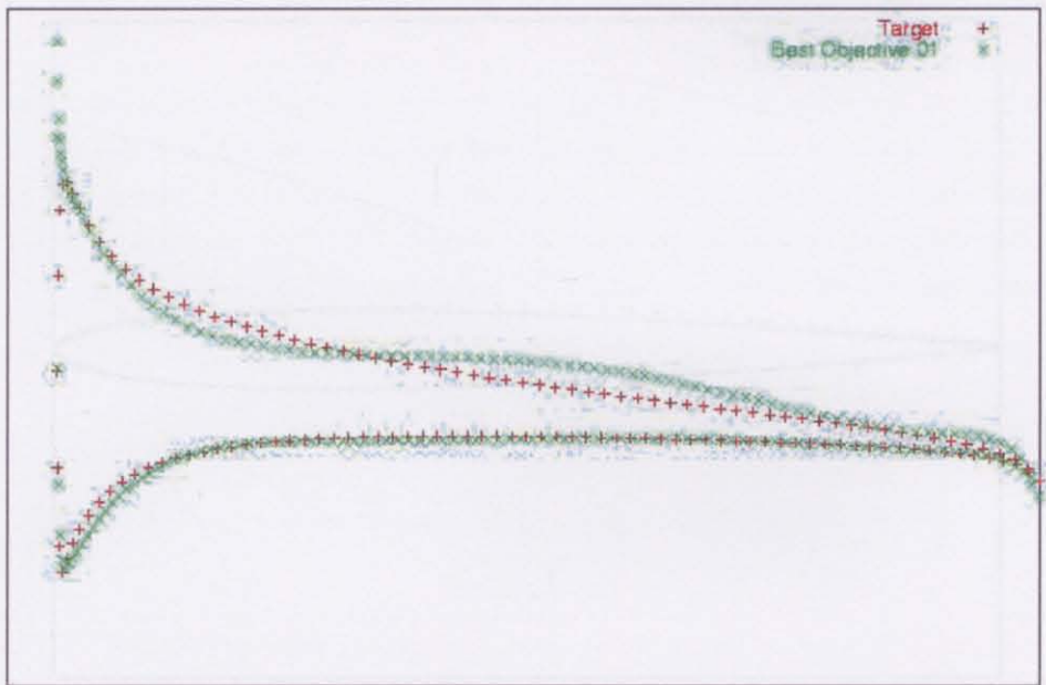
Figure 5.24: Pressure coefficient distribution for objective one.
