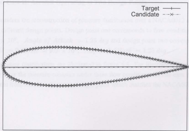
Figure 5.6: Target and computed geometries for single-objective aerofoil pressure coefficient distribution reconstruction problem.
