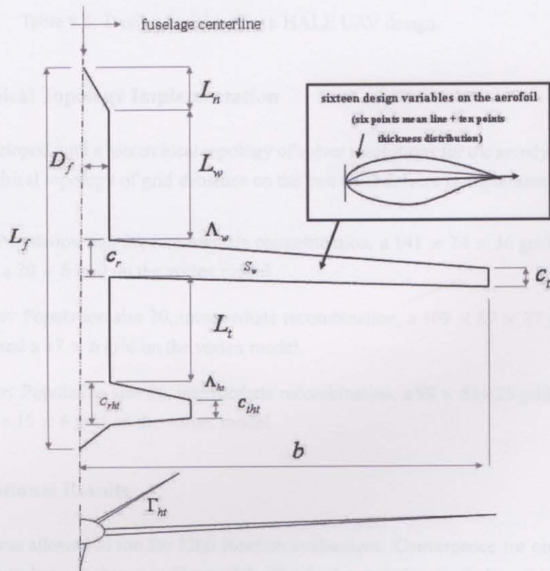
Figure 8.7: Design variables for a HALE UAV design.
