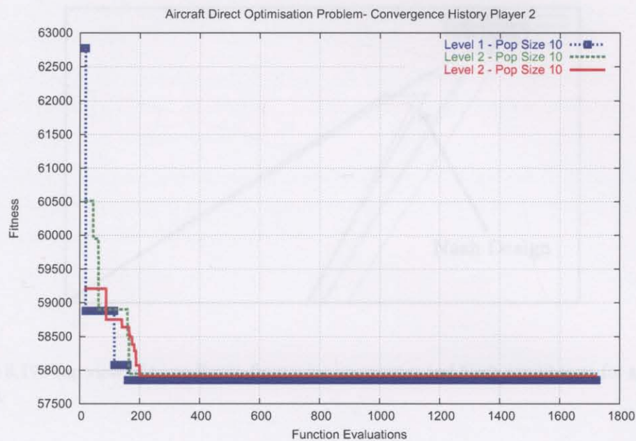
Figure 8.17: Optimisation progress for Player Two.
