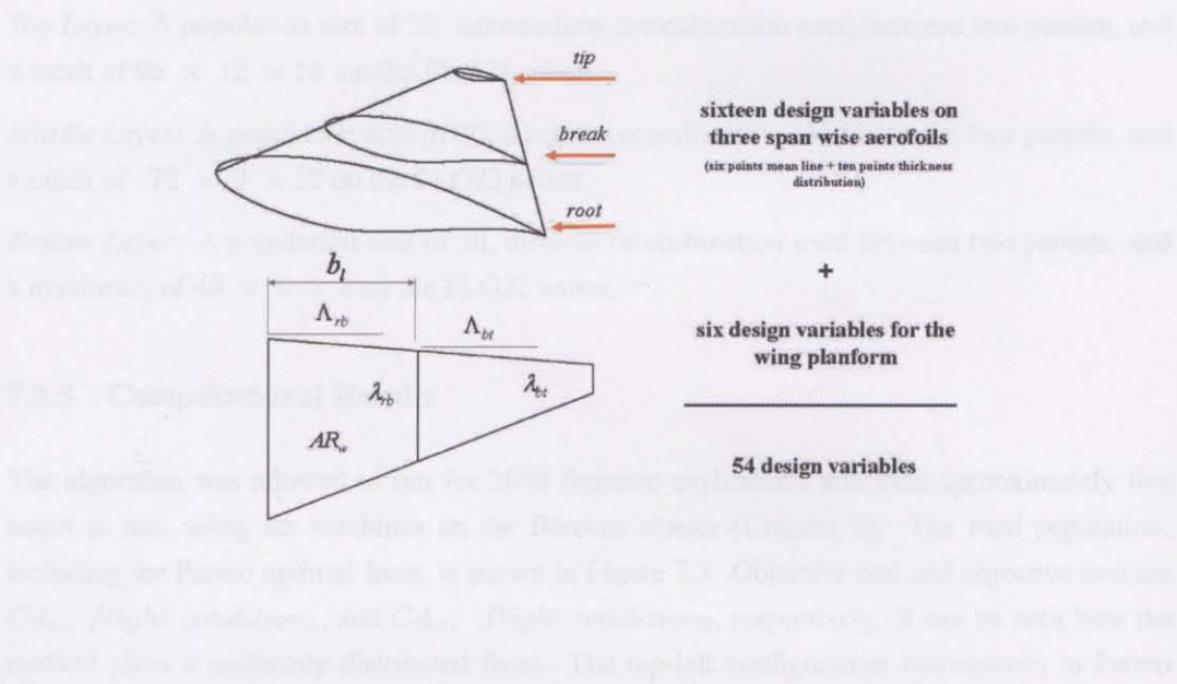
Figure 7.2: Design variables for multi-objective wing design.
