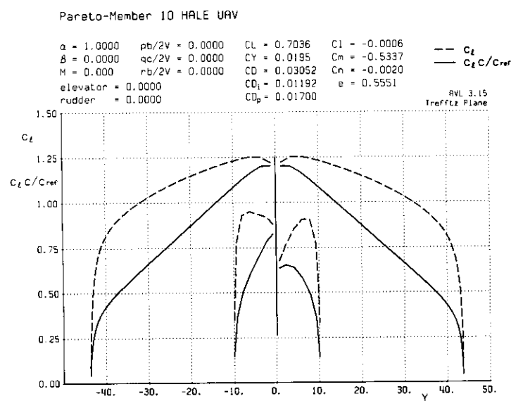
Figure 8.12: Treffitz plane plot for a HALE UAV design – Pareto Member ten.
