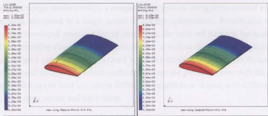
Figure 7.24: Displacement results after structural analysis for wing sampling point four (SP4).
