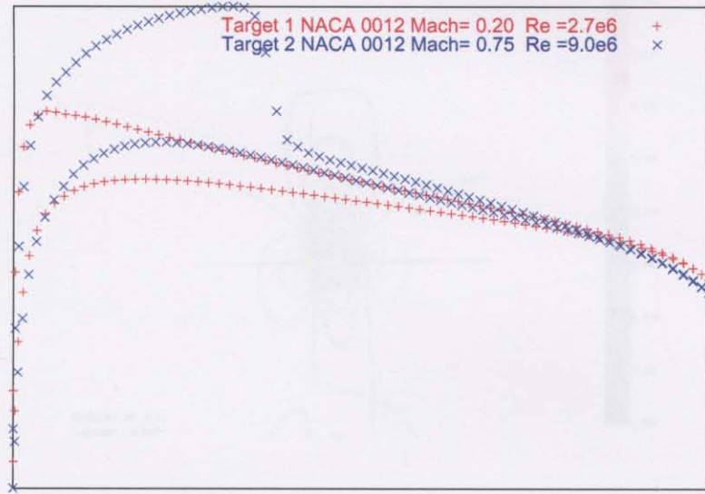
Figure 5.8: Target pressure distributions over NACA 0012 at two flow conditions: M = 0.2 , Re = 2.7 \times 10^6 , Angle of Attack = 1.25 deg and M = 0.75 , Re = 9.0 \times 10^6 , Angle of Attack = 1.25 deg.
