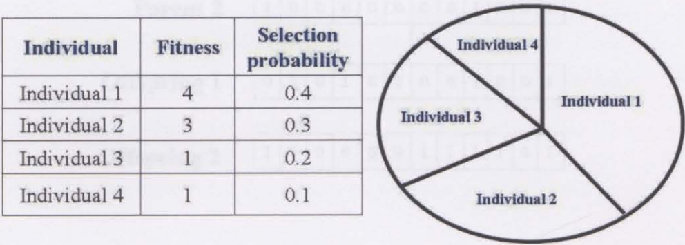
Figure 2.13: Roulette wheel selection.
