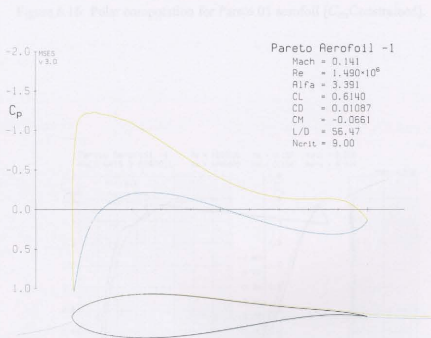
Figure 6.15: Pressure coefficient distribution and aerodynamic data for Pareto 01 for flight condition two [Fast-Cruise] [ C_m Constrained].
