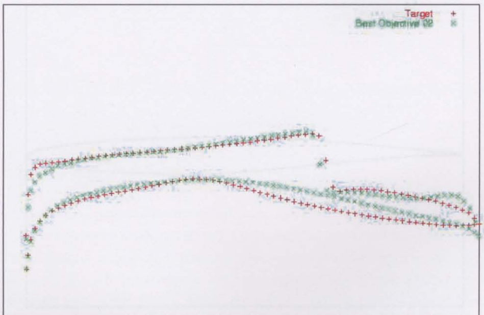
Figure 5.25: Pressure coefficient distribution for objective two.
