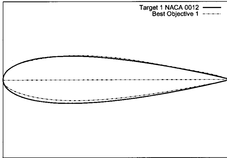
Figure 5.15: Target and computed geometries, multi-point aerofoil design, objective one.
