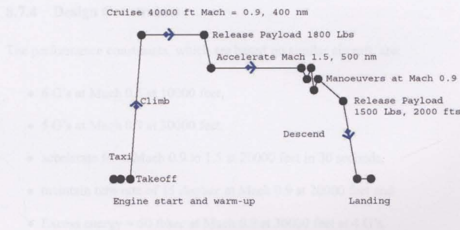
Figure 8.15: Mission profile for a UCAV design.
