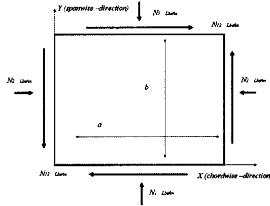
Figure 7.17: Wing cover panel.
