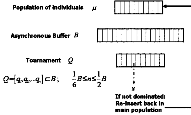
Figure 2.18: Pareto tournament.
