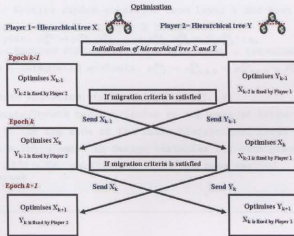
Figure 3.6: Nash HAPEA.
