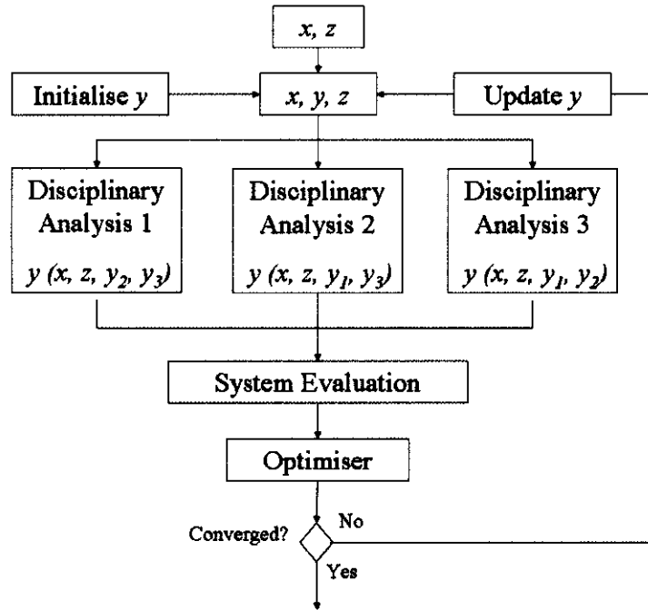
Figure 2.8: Individual Discipline Feasible (IDF).
