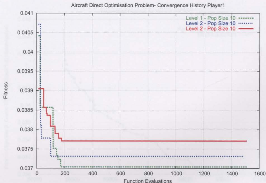
Figure 8.16: Optimisation progress for Player One.
