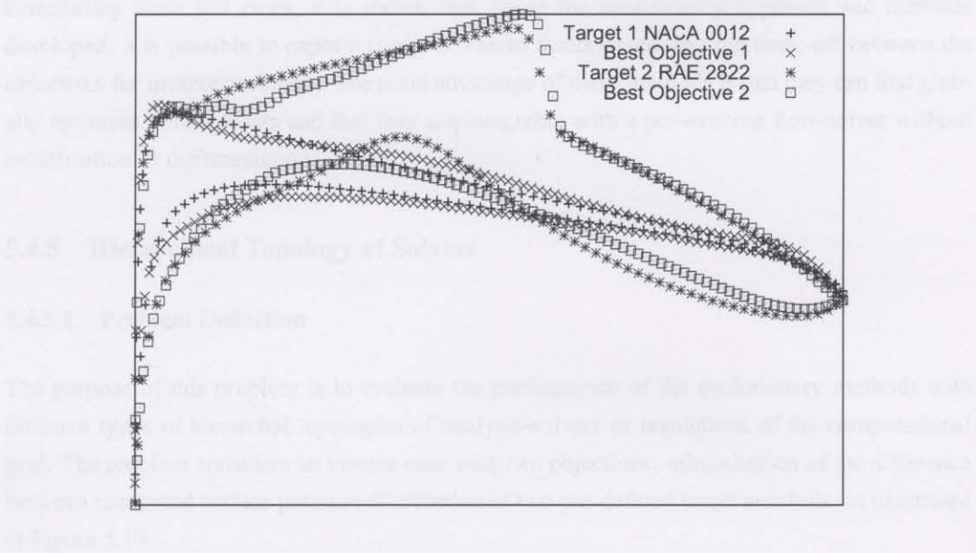
Figure 5.17: Target and computed pressure distribution for multi-point aerofoil design.
