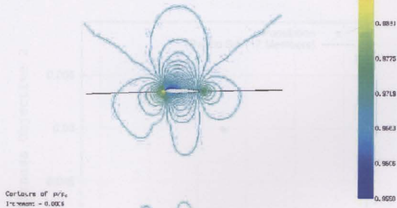
Figure 5.9: Target pressure contours distributions over NACA 0012 at flow conditions: M = 0.2 , Re = 2.7 \times 10^6 , Angle of Attack = 1.25 deg.
