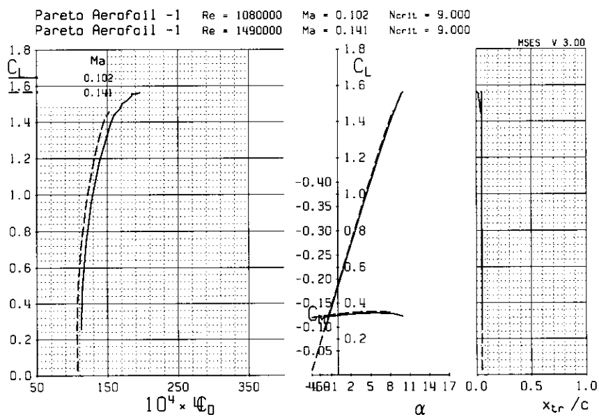
Figure 6.9: Polar computation for Pareto 01 aerofoil [ C_m Unconstrained].
