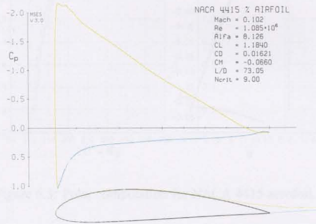
Figure 6.1: Pressure coefficient distribution and aerodynamic data for NACA 4415—flight condition one [Slow-Cruise].
