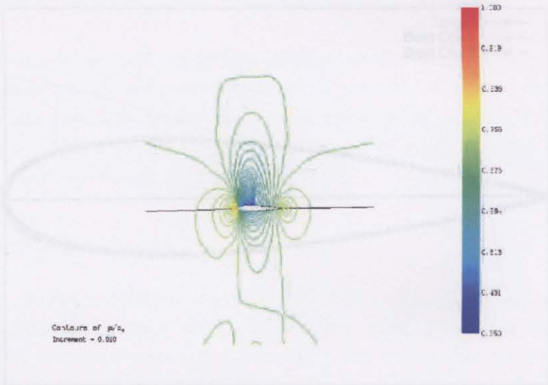
Figure 5.10: Target pressure contours distributions over NACA 0012 at flow conditions: M = 0.75 , Re = 9.0 \times 10^6 , Angle\ of\ Attack = 1.25\ deg .
