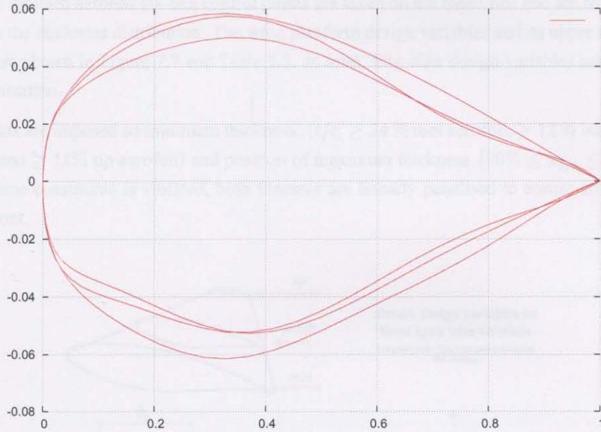
Figure 7.6: UAV wing aerofoil sections for Pareto Member four.
