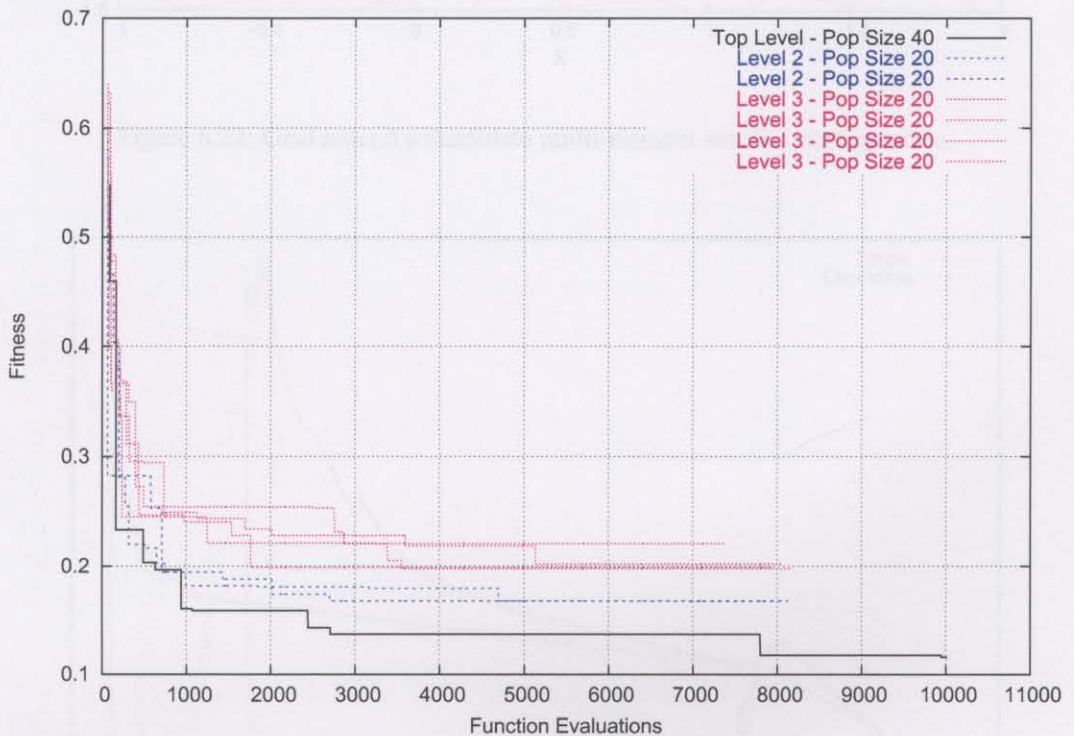
Figure 6.21: Evolution progress for multi-element aerofoil inverse design problem.
