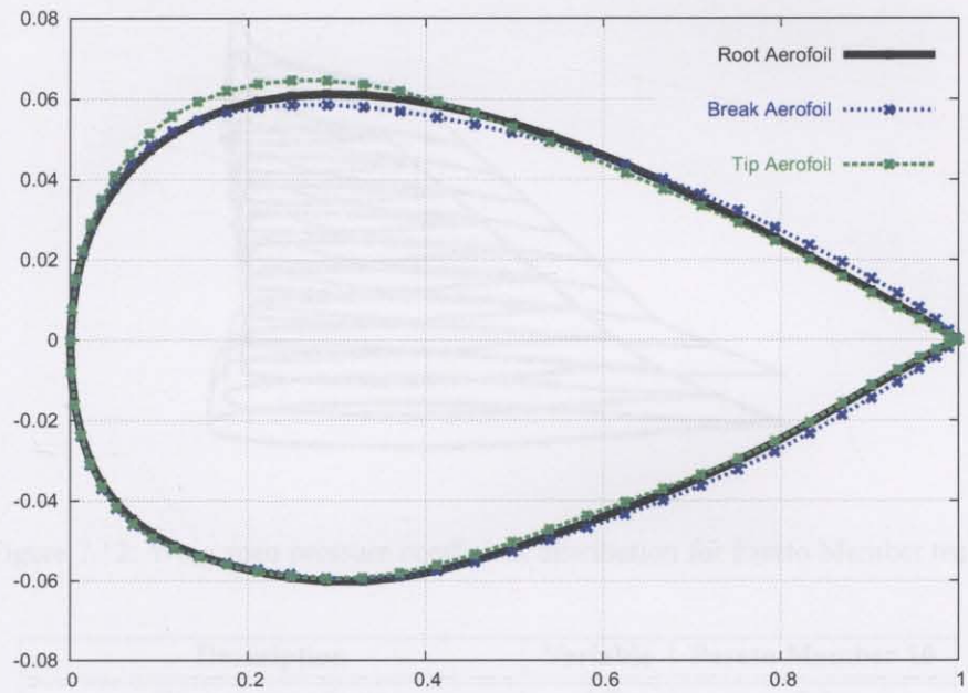
Figure 7.10: Aerofoil sections (root, break and tip) for Pareto Member ten.
