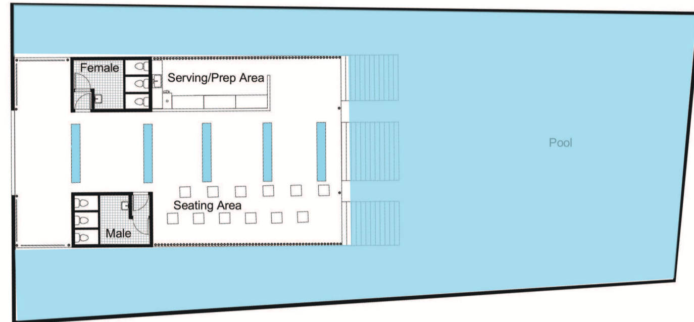
FLOOR PLAN
