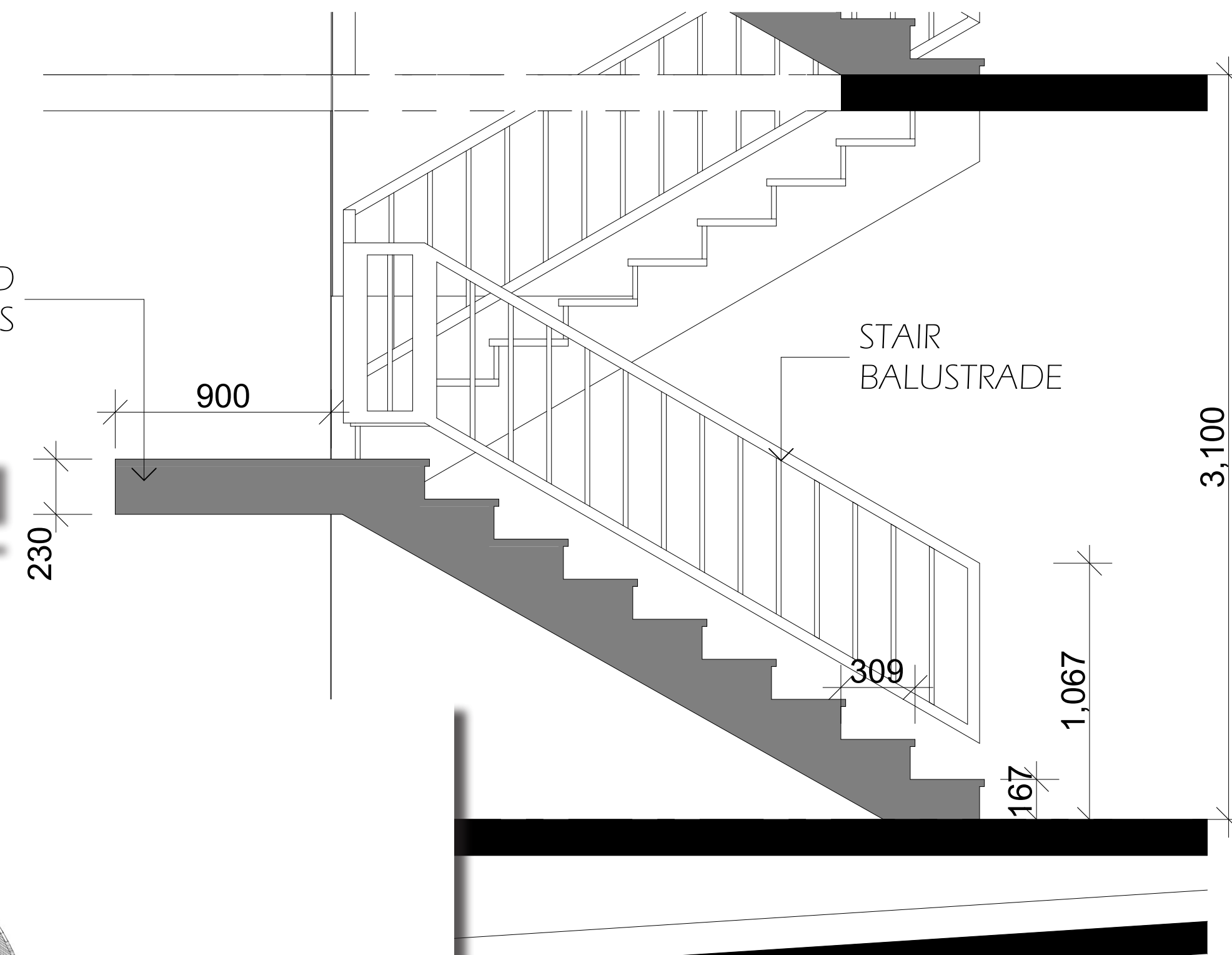
DETAIL SECTION OF STAIRS
