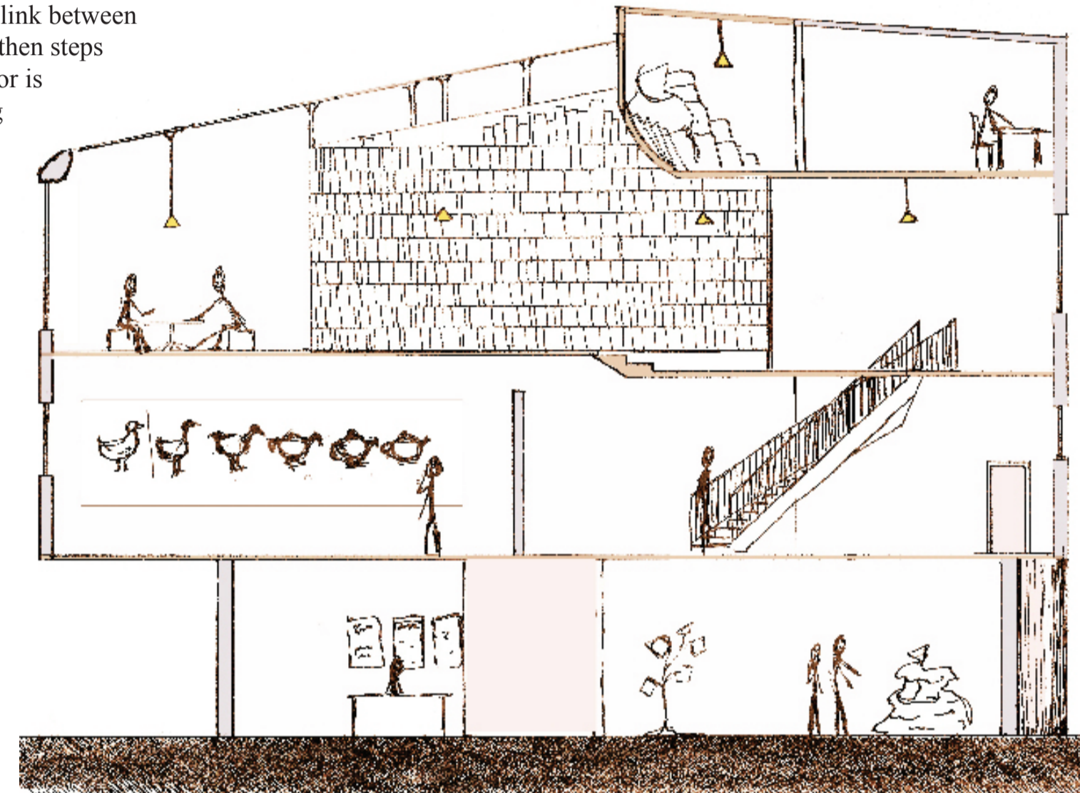
Directly below; section. To the right, from top; elevation (street side), elevation (park side), street entrance to the gallery.
