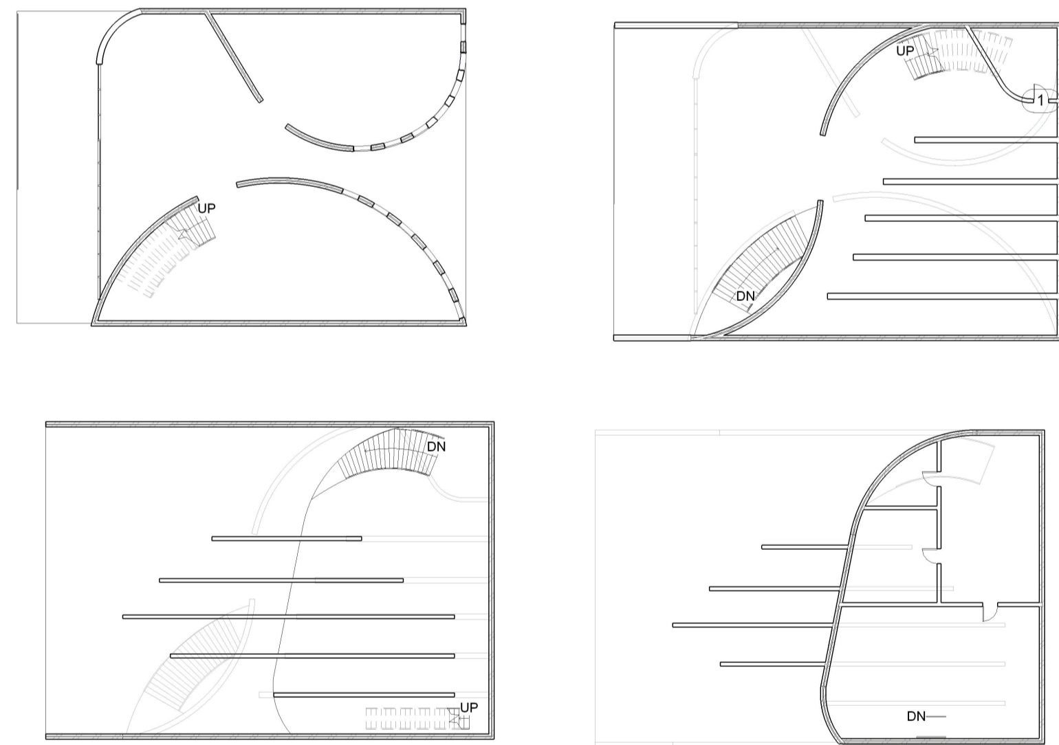
Above; plans (read left to right, ground, first, second, third floor). Below; interior render.
