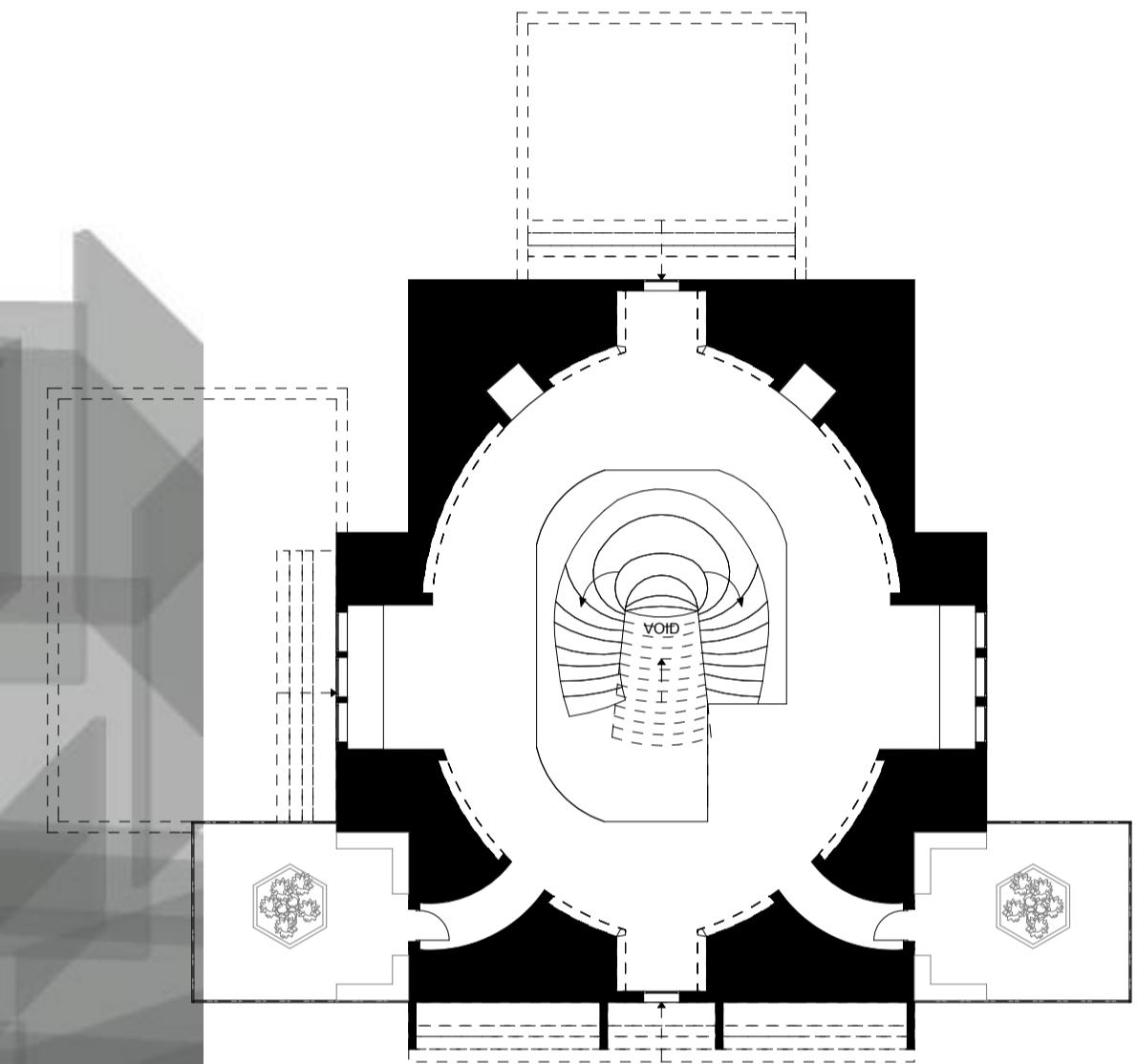
FIRST FLOOR PLAN 1:200
