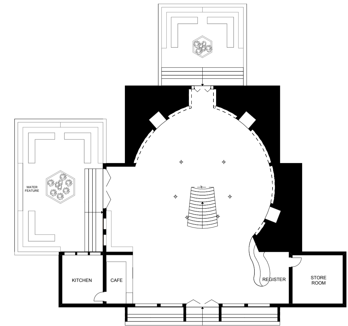
GROUND FLOOR PLAN 1:200
