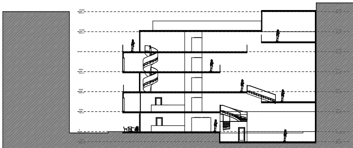
LONG SECTION
