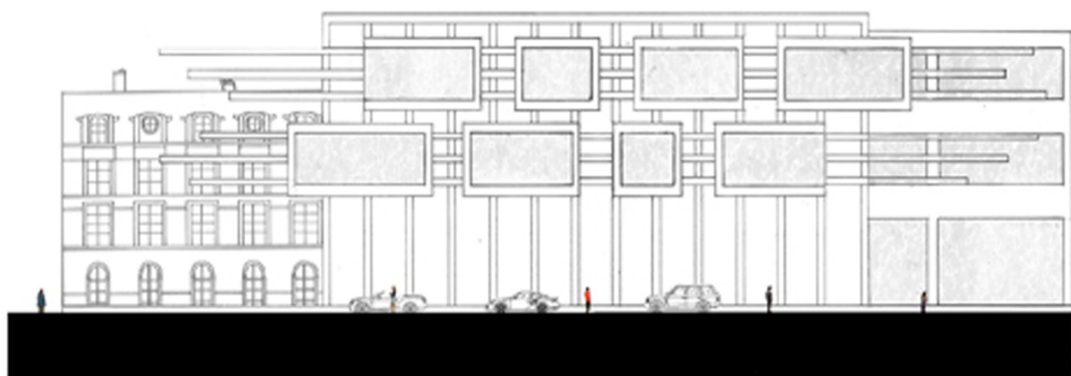
South Elevation 1:200
