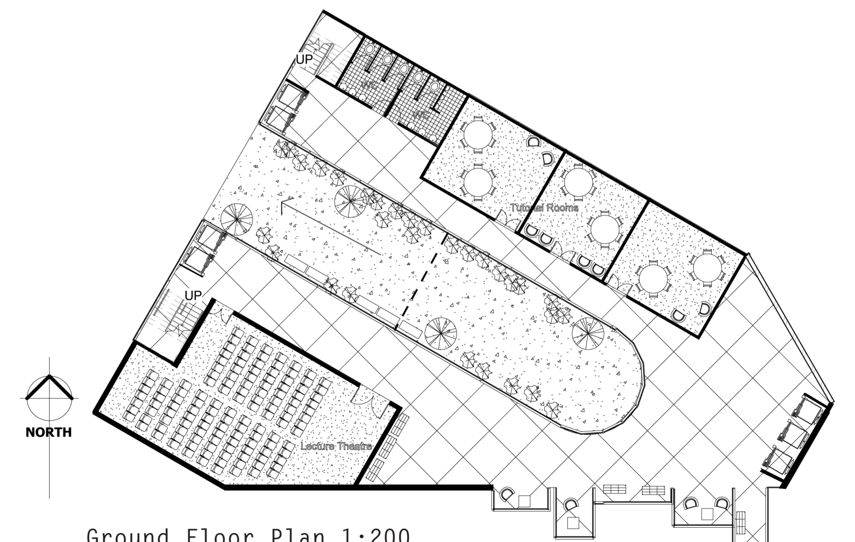
Ground Floor Plan 1:200.
