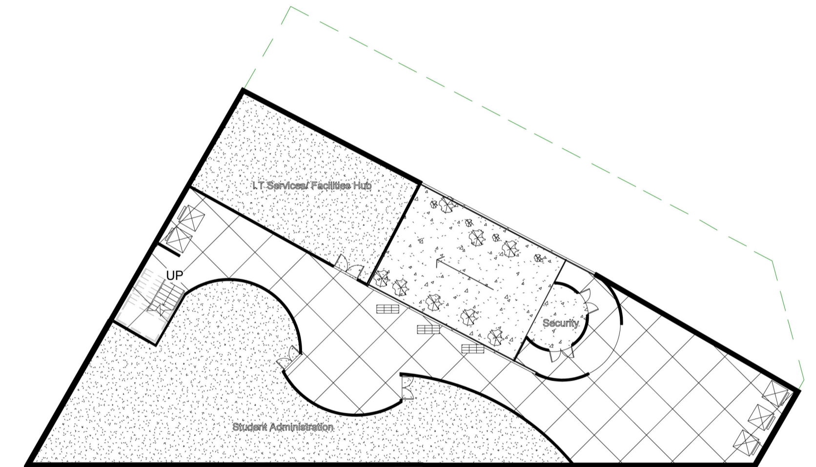
Lower Ground Floor Plan 1:200.
