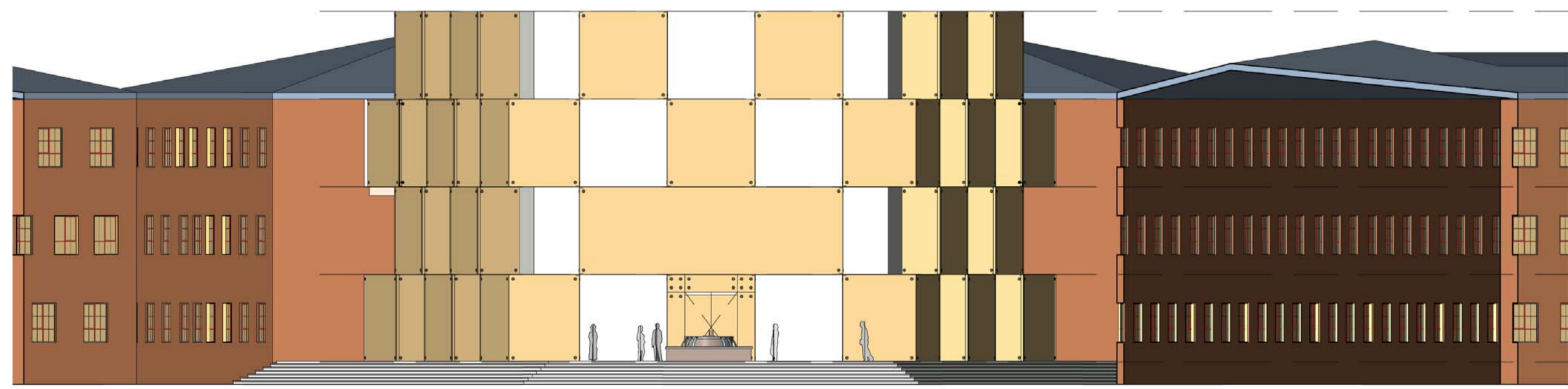
1 South Elevation 1 : 200
