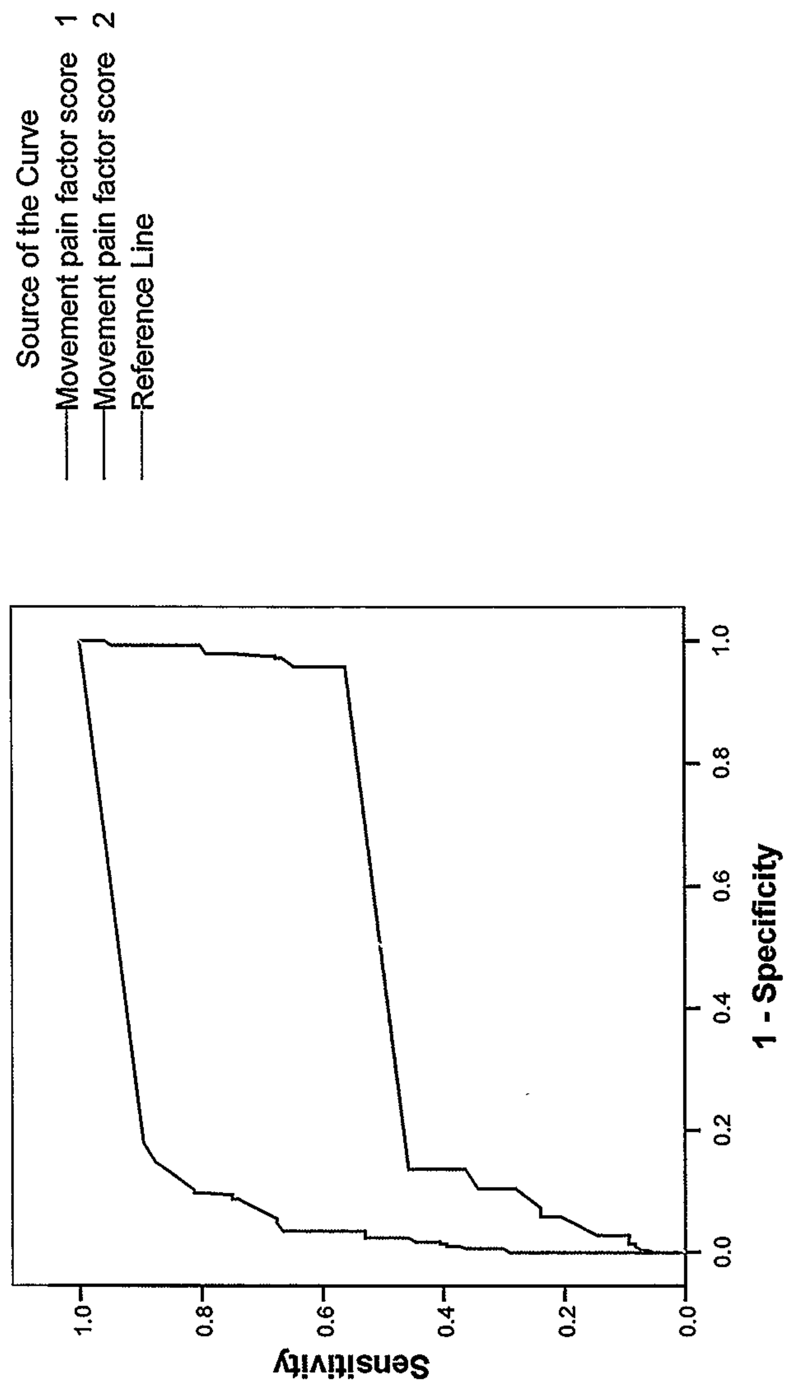
ROC Curve
