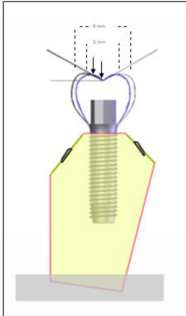
Figure II – 16 Experiment design for an implant-supported single crown with strain gauges attached on buccal and lingual area.
