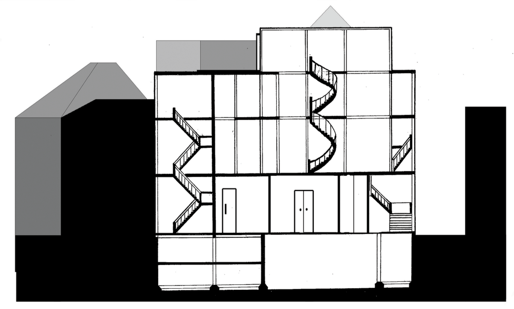
SECTION 1:200
