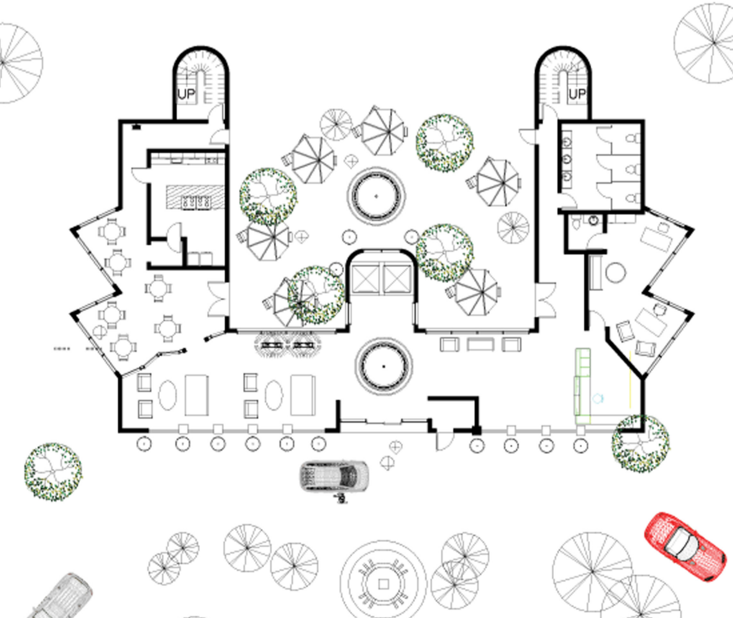
PLANS 1:200
