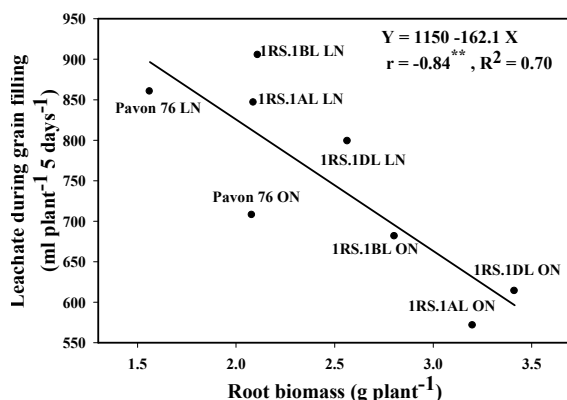
Fig.5. Relationship between the amount of leachate collected in five consecutive days during early grain filling and root biomass per plant for spring bread wheat Pavon 76 and its 1RS translocation lines grown in low level and optimum level of N.
