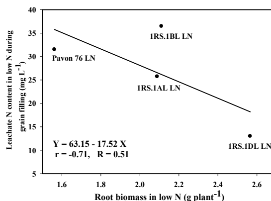
Fig. 6. Relationship between the amount of N in leachate and root biomass per plant during early grain filling for spring bread wheat Pavon 76 and its 1RS translocation lines in low level of N.
