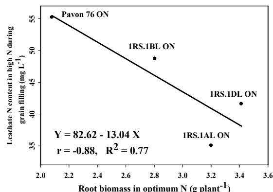
Fig. 7. Relationship between the amount of N in leachate and root biomass per plant during early grain filling for spring bread wheat Pavon 76 and its 1RS translocation lines in optimum level of N.
