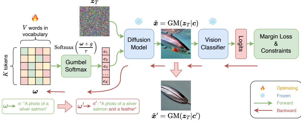
FIGURE 1.1. The overall pipeline of our attack method. The selection of words is relaxed to be differentiable by using a Gumbel Softmax with temperature \tau . When \tau \rightarrow 0 , the Gumbel Softmax outputs exhibit proximity to one-hot vectors while retaining differentiability. After an image is generated, a CLIP [18] classifier and a margin loss are employed to optimize \omega aiming to generate images that cannot be correctly classified by CLIP.
