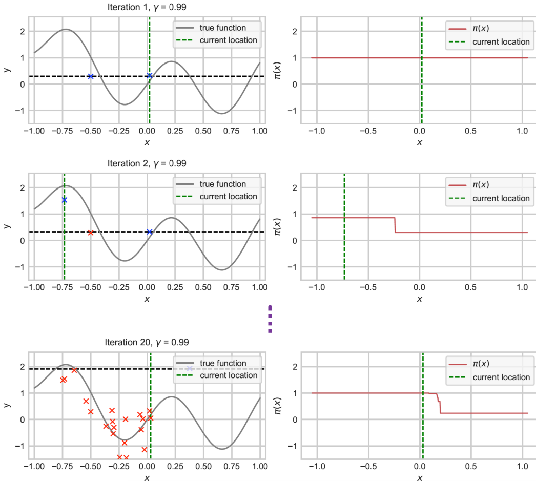
FIGURE 5.3. BORE iterations when \gamma = 0.99 .
