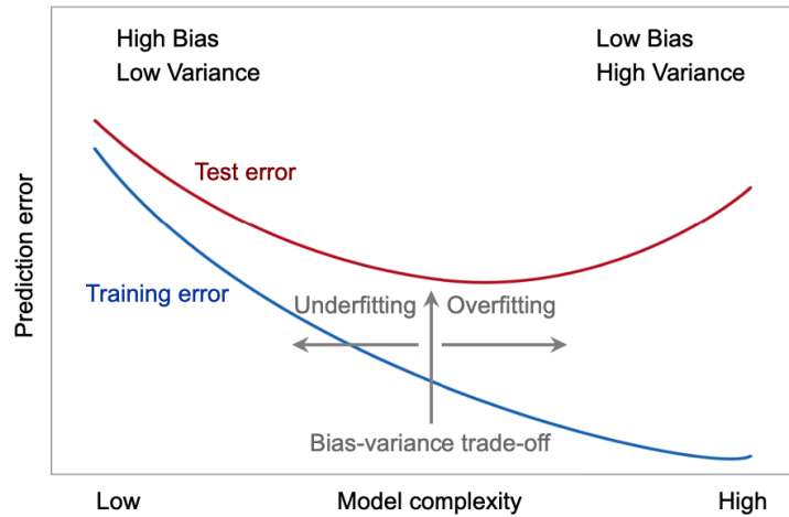
FIGURE 2.7. Bias and variance trade-off, and the behavior of training error (blue curve) and test error (red curve) as the predictive model complexity increases. The training and test errors correspond to the errors obtained by evaluating training and test data with the predictive model respectively.
