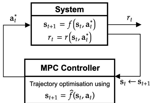
FIGURE 3.1. MPC controller diagram where the output signal is the reward.
