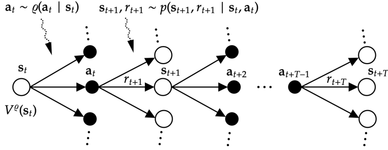
FIGURE 2.21. States and interactions sampled by an MDP. V^{\varrho}(s_t) is the value at state s_t , and \varrho(a_t|s_t) is a stochastic policy.
