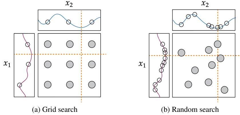
FIGURE 2.10. Search space coverage for grid search and random search.
