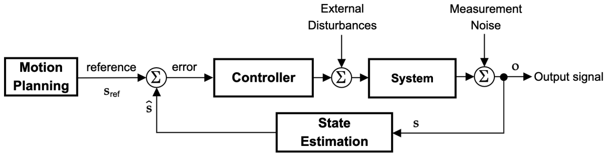
FIGURE 2.2. Typical components and variables in control system design.
