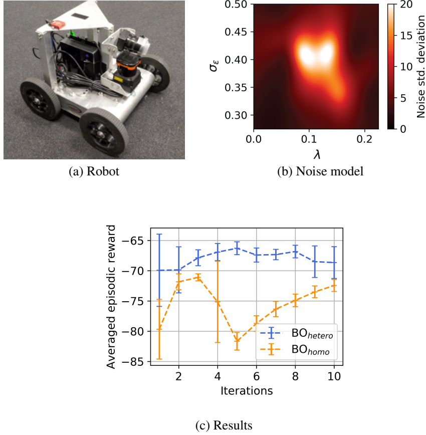
FIGURE 3.11. (a) Experiments with a physical robot known as Wombot, (b) the learnt heteroscedastic noise model and (c) the resulting performance for each BO method. The results were averaged over 3 independent trials for each algorithm, totalling 60 runs of MPPI in 20-second episodes on the robot.
