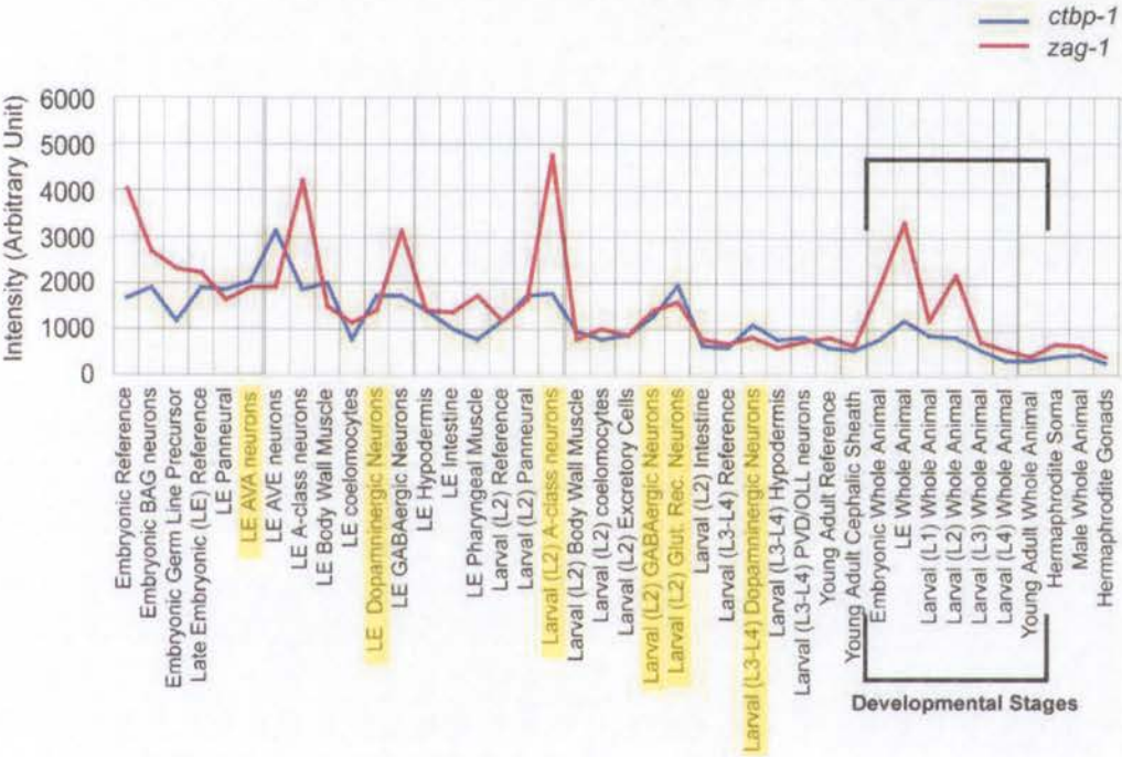
Figure 3.7: ctbp-1 and zag-1 show a similar expression pattern throughout development and enrichment in the same type of tissues. The graph shows relative expression intensity of ctbp-1 and zag-1 plotted against the tissue types and developmental stages. The data are obtained from a website Wormviz which includes results from a recently published paper on a C. elegans gene expression map (Spencer et al., 2011). The intensity of expression is determined by normalisation of expression levels of each gene in the relevant tissue against an appropriate reference samples. For instance, for embryonic stage the reference is Embryonic Reference. Embryonic neurons that are cultured overnight are called late embryonic and the reference for these data sets is Late Embryonic
