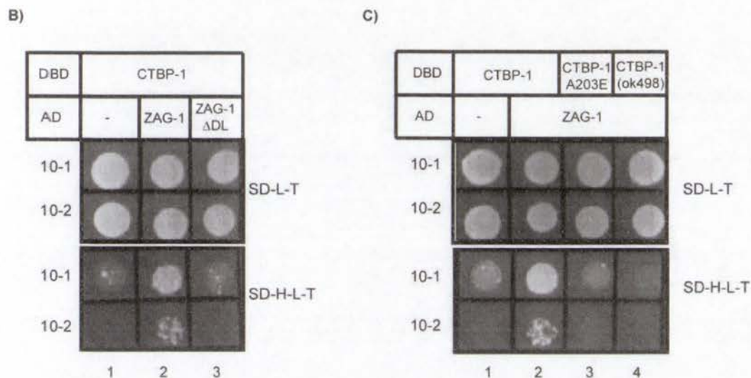
Figure 3.6: CTBP-1 interacts with neuronal transcription factor ZAG-1. A) A yeast two hybrid screen for proteins that interact with nematode CTBP-1 identified a partial cDNA encoding residues 580-747 of murine \delta EF1 (upper and middle panels). The nematode homologue of murine \delta EF1 is ZAG-1 (lower panel). Zinc finger domains are shown in blue, homeodomains are shown in black, and putative CtBP interaction motifs are shown by dashed lines. B and C) Yeast two-hybrid assays were performed to examine the interaction of CTBP-1 with ZAG-1. The assays were performed by fusing the test proteins to the C-terminus of either the Gal4 DNA binding domain (DBD) or the Gal4 activation domain (AD). Transformants were selected on SD-L-T plates. Colonies were picked from these plates and incubated overnight in liquid SD-L-T media. The cultures were normalised to an OD600 of 1 and serial dilutions were made. 10 \mu l was then pipetted on to SD-L-T plates and SD-H-L-T, which were incubated at 30 ^{\circ} C for 72 hours. Growth on SD-H-L-T plates is indicative of a physical interaction between the test proteins. The interaction of CTBP-1 and ZAG-1 was assessed (B column 2). The PXDLS-like motif in ZAG-1 was mutated and the mutant protein (ZAG-1 \Delta DL) was tested for its capacity to interact with CTBP-1 (B column 3). The dependence of the interaction between CTBP-1 and ZAG-1 on the PXDLS-binding cleft of CTBP-1 was assessed by mutating one residue within the putative PXDLS-binding cleft and testing the
