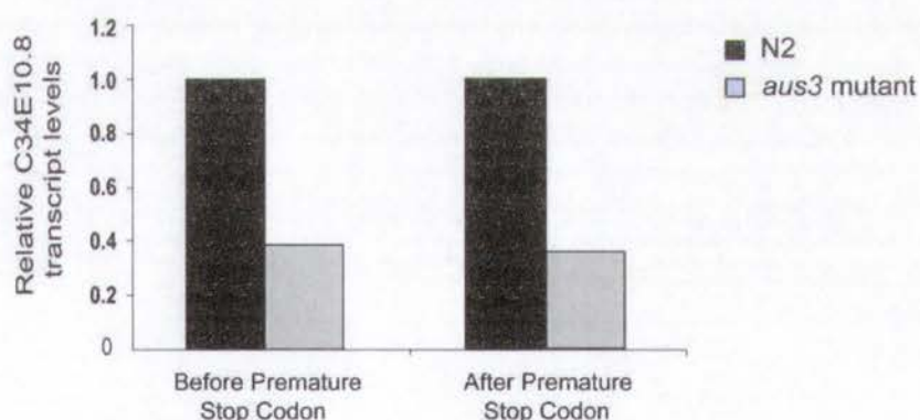
Figure 5.5: The premature stop codon in aus3 mutants might lead to production of a truncated protein and degradation of the C34E10.8 transcript via non-sense mediated decay (NMD). A) The gene model for C34E10.8 and the position of the premature stop codon in aus3 mutants is indicated. The nonsense mutation in the aus3 allele is in the middle of the 15 th exon and it is 109 nucleotides apart from the 14/15 exon-exon junction. Exons are shown as blue boxes and introns are indicated as black lines. B) The amino
