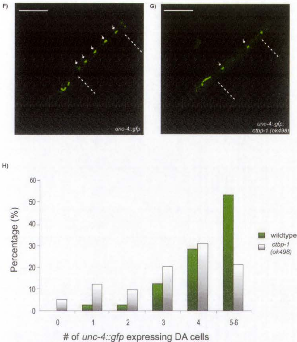
Figure 3.3: ctbp-1(ok498) mutants show defects in DA class neurons. A) The schematic shows Ventral Nerve Cord motor neurons of a hermaphrodite at the L1 stage. (Adapted from Sulston et al. , 1983). The analysed region is indicated with dashed lines. For markers ACR-5::YFP and UNC-4::GFP the analysed region resides between the neurons in the head, termed the retrovesicular ganglion, to the neurons in the tail termed the pre-anal ganglion. However, for the UNC-25::GFP marker, the DD6 cell in the pre-anal ganglion is included in the analysis B) Representative images show a hermaphrodite at the L1 stage expressing the ACR-5::YFP marker in wild type C) and ctbp-1(ok498) mutant background. Neurons DB3-DB7 are marked (◆). D) Representative images show a hermaphrodite at L1 stage expressing UNC-25::GFP in wild type E) and ctbp-1(ok498) mutants background. Neurons corresponding to DD2-DD6 are marked (◆). n=50 for both ACR-5::YFP and UNC-
