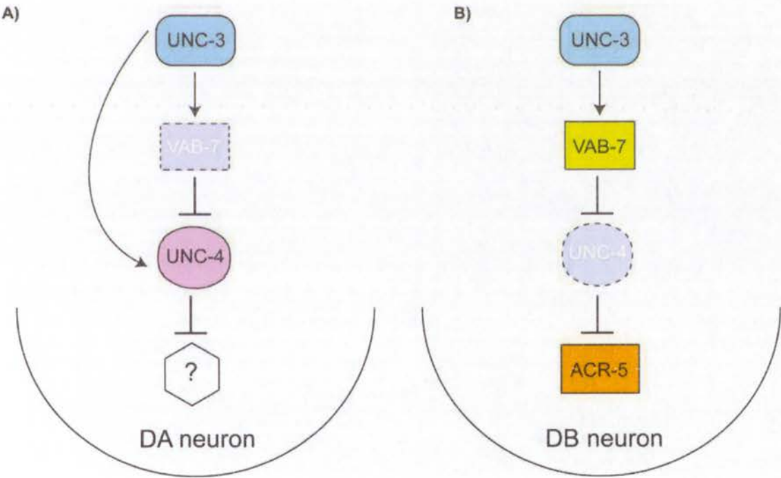
Figure 3.9: The UNC-3 transcription factor works as a terminal selector in embryonically derived cholinergic DA and DB neurons. A) UNC-3 activates UNC-4 and indirectly represses DB type traits in DA
