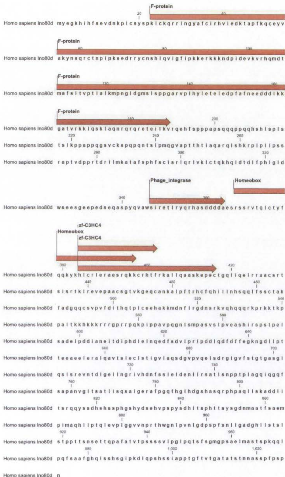
Appendix Figure 3: The predicted domain structure of human INO80d. The predicted domains were obtained through the software Workbench. According to this prediction, human INO80d has a putative F-protein
