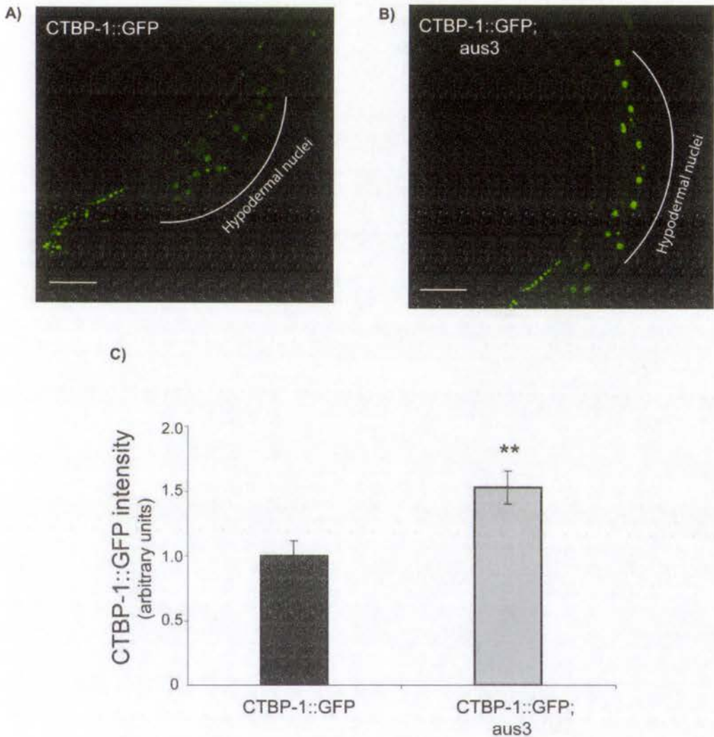
Figure 5.2: Mutant animals carrying the aus3 allele showed elevated levels of CTBP-1::GFP expression in the hypodermis. Representative images of A) CTBP-1::GFP expression in wildtype background B) and CTBP-1::GFP expression in aus3 mutant background are shown. Hypodermal nuclei are indicated. Anterior is to the left, scale bar shows 50 \mu m. C) Graph comparing CTBP-1::GFP expression intensity in the hypodermis of wild type and aus3 mutant animals. The anterior region of transgenic animals in wild type and aus3 mutant background were imaged and the expression level of CTBP-1::GFP was quantified using ImageJ software with the same capture settings for all conditions (i.e, laser intensity, voltage and gain power). The graph presents
