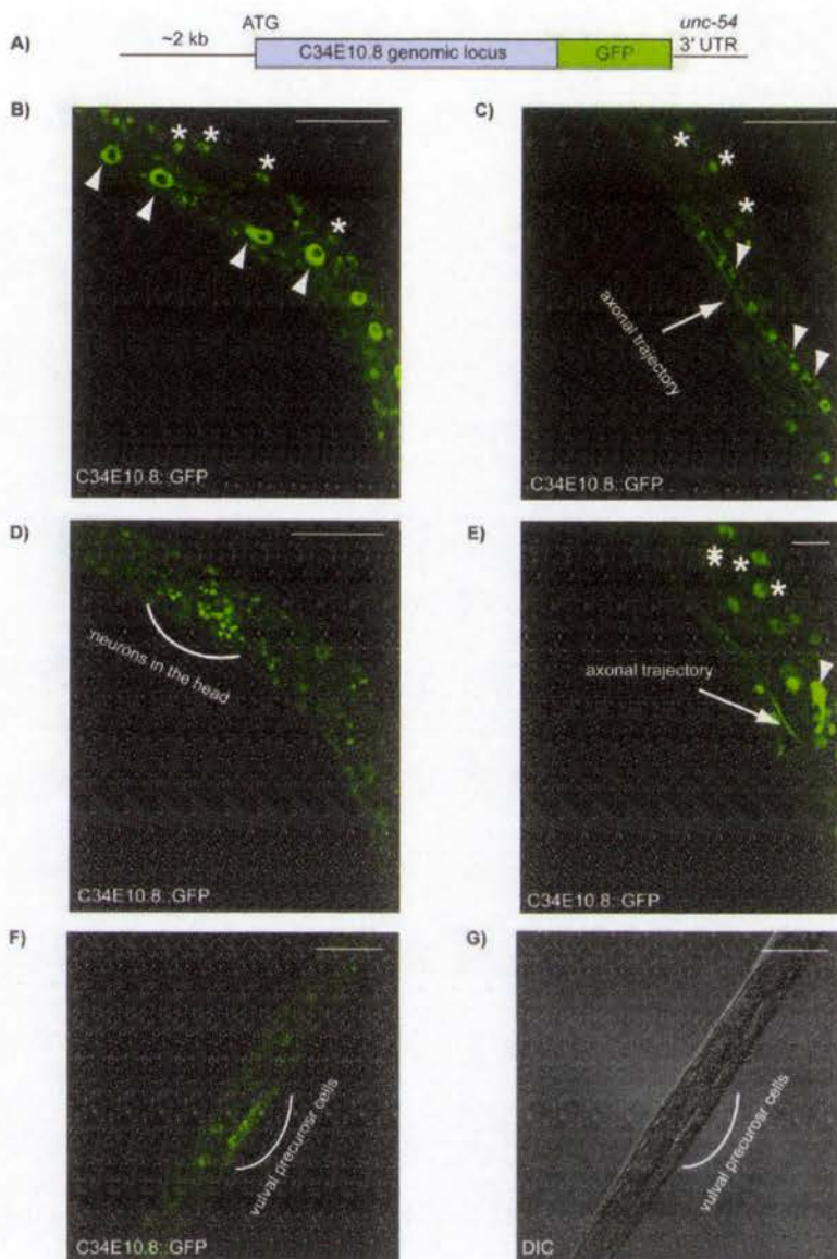
Figure 5.6: C34E10.8 is expressed in many somatic cells. A) The reporter construct carrying the entire coding sequence of full length genomic C34E10.8 with its 2kb promoter was used to generate a transgenic animal expressing C34E10.8::GFP fusion protein for expression pattern analysis. To aid expression of the fusion template the unc-54 3' UTR was used. Analysis of transgenic animals at adult stage has shown that C34E10.8::GFP expression is detected in various tissues. Identification of cells is based on the anatomy of the nematode, morphology of the cells and the size of the nucleolus. B) Expression of C34E10.8::GFP is observed in hypodermal cells (indicated as *) and in the intestinal cells (indicated with arrow heads). C) Expression of
