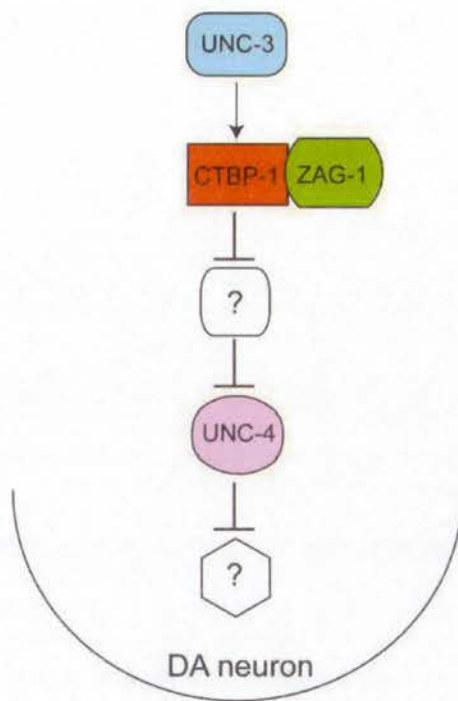
Figure 3.10: A model of how CTBP-1 and ZAG-1 might regulate specification of DA neurons. CTBP-1 might be activated by UNC-3 and by some mechanism activate UNC-4 activities in the DA neurons. This could be via an adaptor protein that works as an UNC-4 repressor. In this scenario, CTBP-1 inhibits expression of a novel UNC-4 repressor via interaction with ZAG-1 and this way indirectly activates UNC-4. UNC-4 activity is required for correct expression of terminal differentiation genes. CTBP-1 and ZAG-1 might therefore indirectly regulate expression of these genes.
