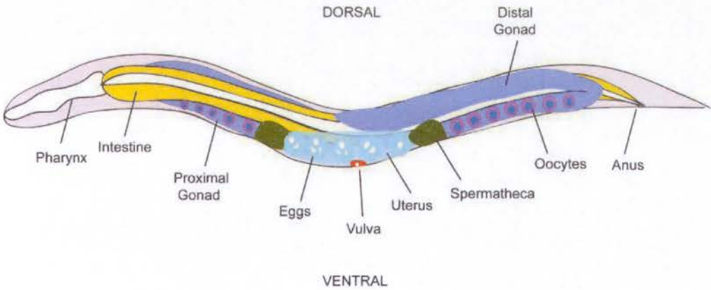
Figure 1.3: Basic anatomy of C. elegans at adult stage. Adapted from Varki et al. (Varki et al., 2009.)
