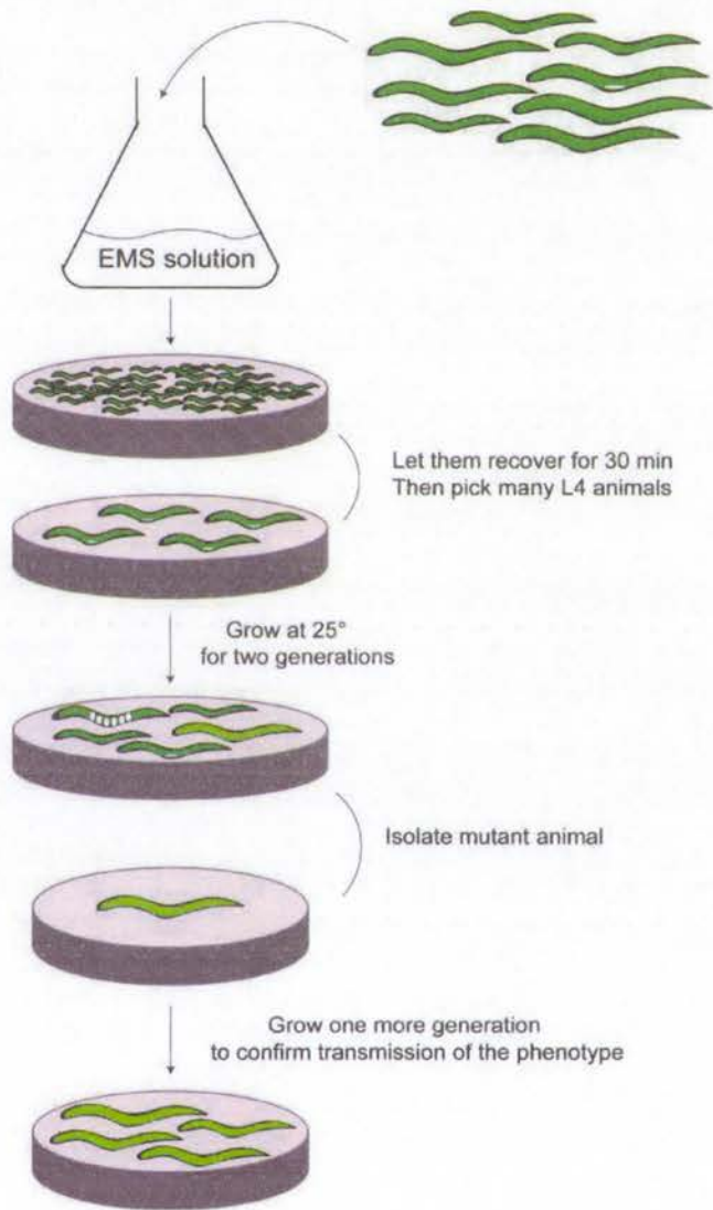
Figure 5.1: Mutagenesis of ctbp-1::gfp transgenic animals. A mixed population of animals was treated with Ethyl Methane Sulfonate (EMS), washed and allowed to recover for half an hour. After mutagenesis, animals at
