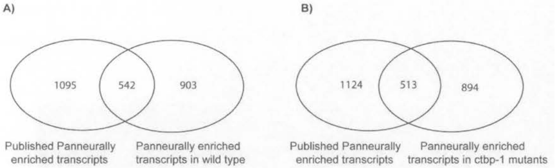
Figure 4.3: Pan-neurally enriched transcripts correlate with the published list. Pan-neurally expressed genes with fold change of \geq 2 and adjusted p-value of \leq 0.05 were compared with the published pan-neurally enriched data. The pan-neurally enriched transcripts in wild type samples (A) and in ctbp-1(ok498) mutant samples (B) show considerable overlap with the published (Von Stetina et al., 2007) pan-neurally enriched transcripts.
