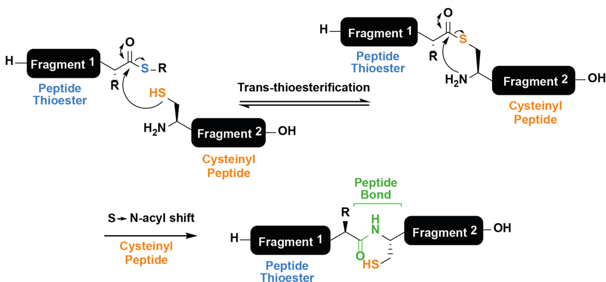
Figure 1: Mechanism of Native Chemical Ligation (NCL). The reaction between peptide thioester and cysteinylyl peptide fragments via an initial trans-thioesterification followed by an S → N acyl shift to afford a native peptide (amide) bond.
