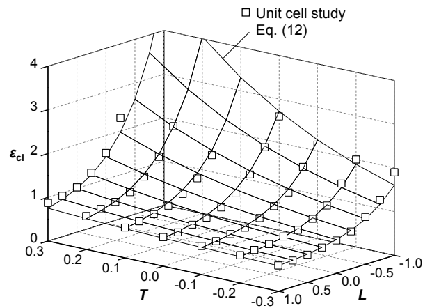
Fig. 9 Critical strain in low triaxiality
