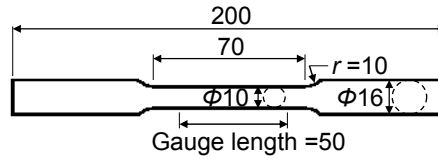
Fig. 1 Geometries of SRB coupon (unit: mm).
