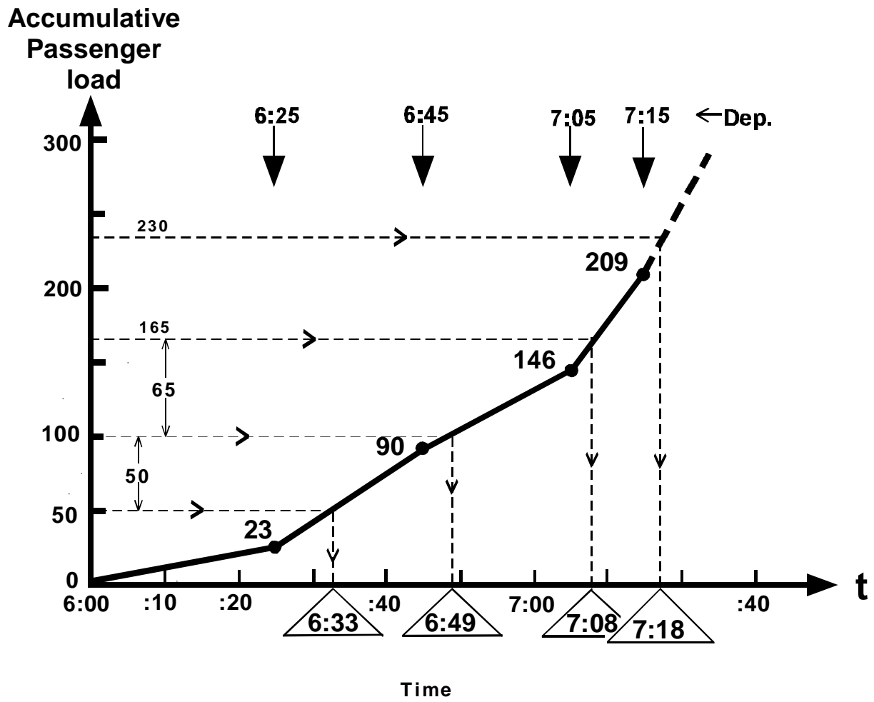
Fig. 4 Accumulative Passenger Load Curve using Level 2 Analysis
