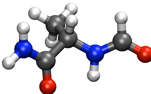
Figure 1.2: Model of peptide backbone containing an alanine residue that was used in the bond dissociation energy study of Rauk and co-workers. 34 (key: grey = C, white = H, blue = N, red = O).
