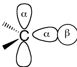
Figure 2.1: Spin Polarization in the Methyl Radical.
