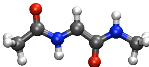
(a) \text{CH}_3\text{CONH}\text{--}\bullet\text{CH}\text{--}\text{CONHCH}_3
