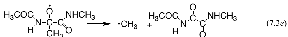
Figure 7.3: Five model peptides for the study of the \beta -scission of the C–R side-chain bond from an \alpha -C-centered alkoxy radical.
