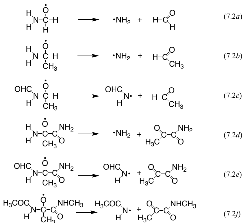
Figure 7.2: Six model peptides for the study of the \beta -scission of the C–N backbone bond from an \alpha -C-centered alkoxy radical.
