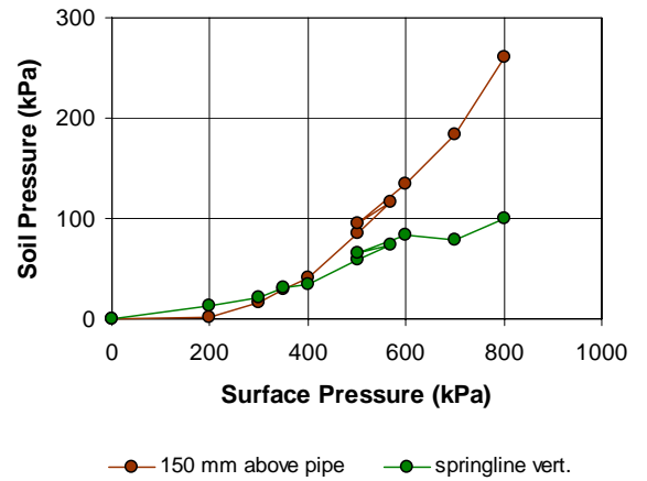
d) Test 450/5, 800 mm of cover
