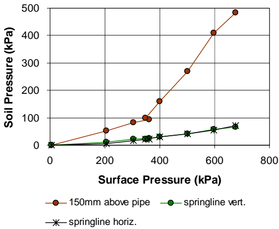
c) Field test F450/3, 600 mm of cover
