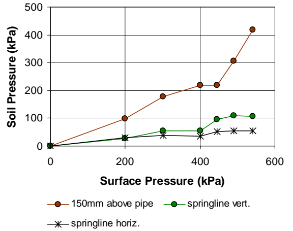
b) Test 450/2, 450 mm of cover
