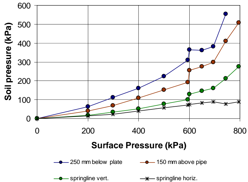
b) Test 375/8 with 700 mm of cover
