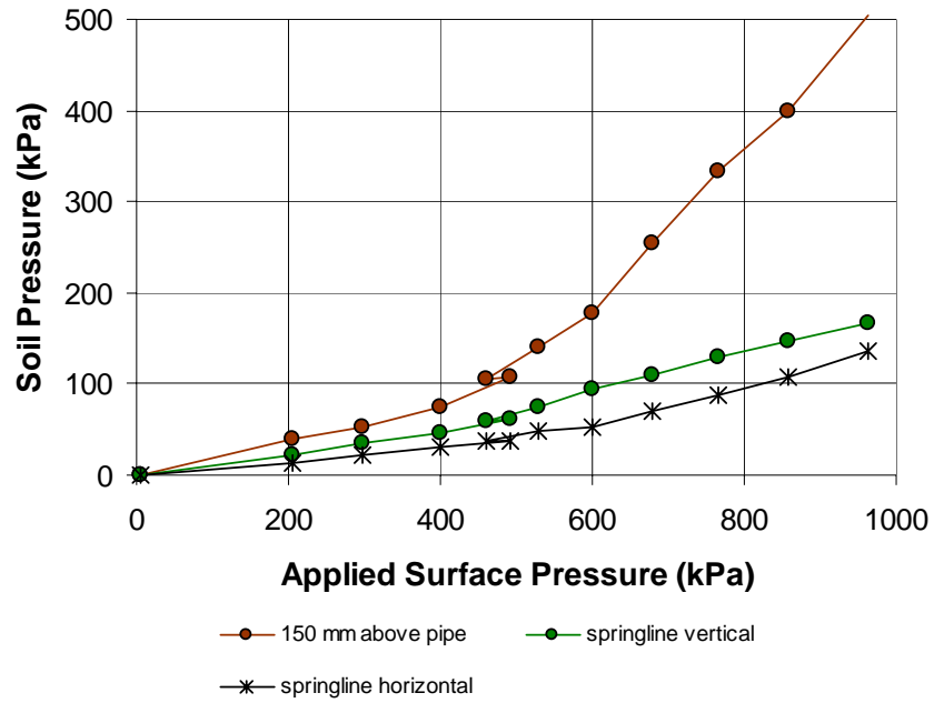
a) F375/7, field test with 700 mm of cover
