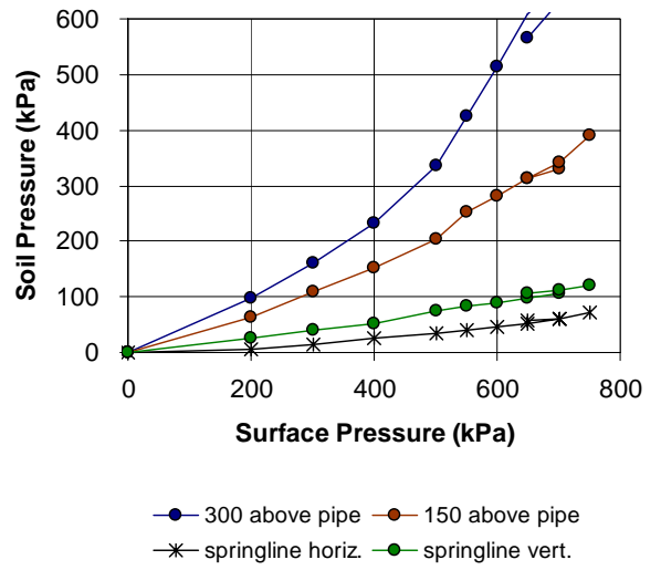
e) Test 300/8, 110VX, 650 mm of cover
