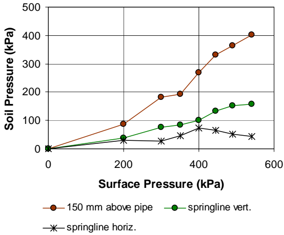
a) Test 450/1, 450 mm of cover
