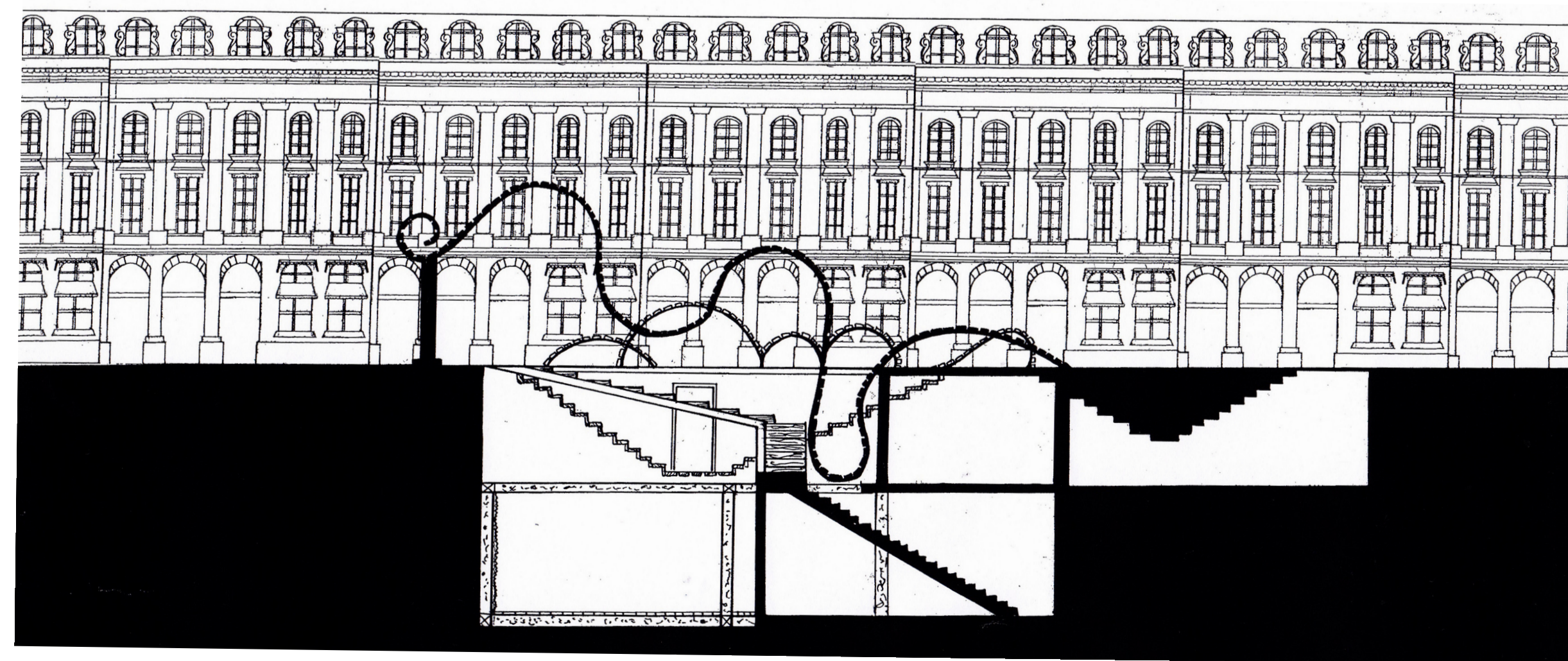
Section Scale 1:200
